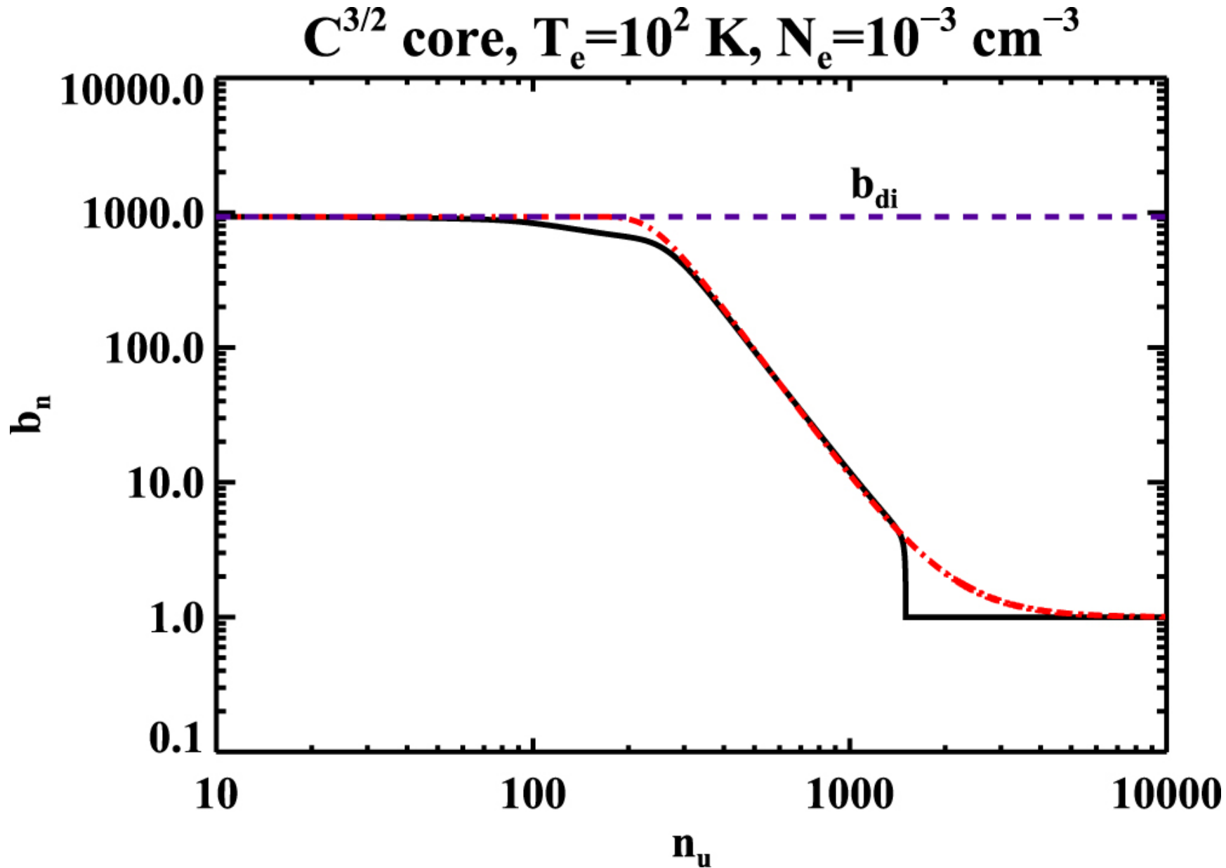
Figure 7. from Low-frequency Carbon Radio Recombination Lines. I. Calculations of Departure Coefficients null 2017 APJ 837 141 doi:10.3847/1538-4357/aa5d9e https://dx.doi.org/10.3847/1538-4357/aa5d9e © 2017. The American Astronomical Society. All rights reserved.
