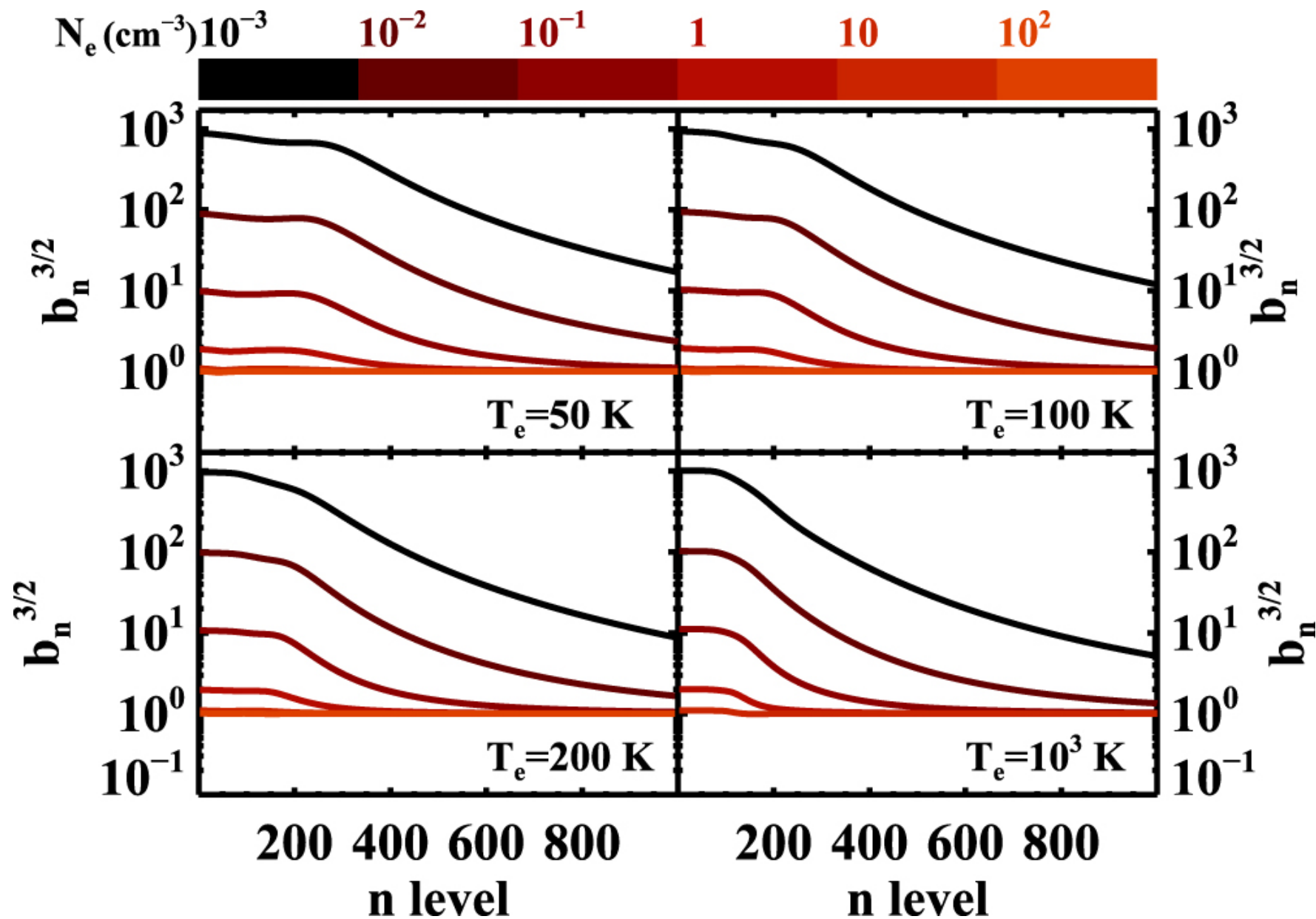
Figure 5. from Low-frequency Carbon Radio Recombination Lines. I. Calculations of Departure Coefficients null 2017 APJ 837 141 doi:10.3847/1538-4357/aa5d9e https://dx.doi.org/10.3847/1538-4357/aa5d9e © 2017. The American Astronomical Society. All rights reserved.
