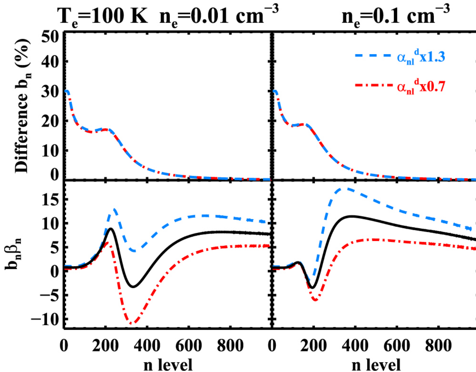
Figure 16. from Low-frequency Carbon Radio Recombination Lines. I. Calculations of Departure Coefficients null 2017 APJ 837 141 doi:10.3847/1538-4357/aa5d9e https://dx.doi.org/10.3847/1538-4357/aa5d9e © 2017. The American Astronomical Society. All rights reserved.
