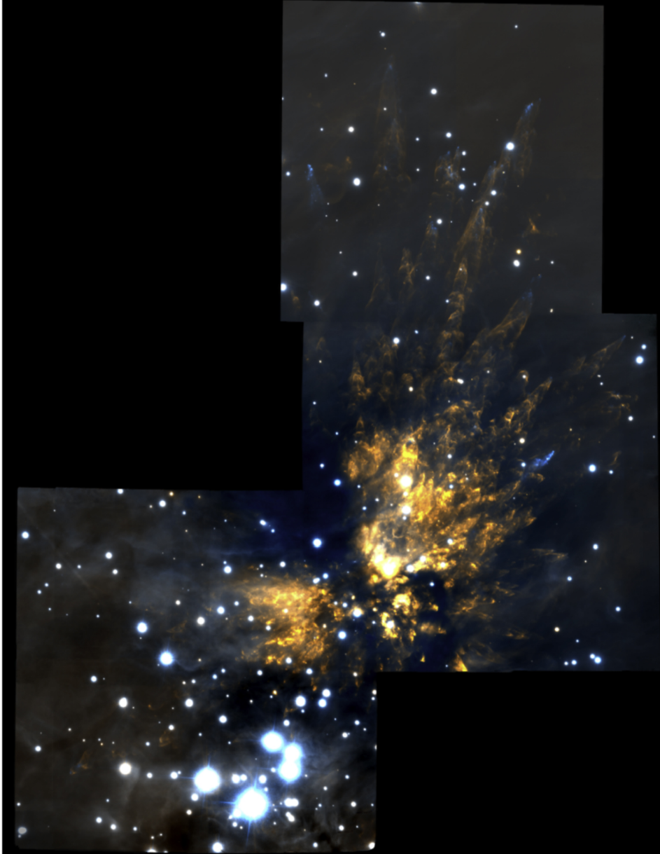
Figure 9. from The ALMA View of the OMC1 Explosion in Orion null 2017 APJ 837 60 doi:10.3847/1538-4357/aa5c8b https://dx.doi.org/10.3847/1538-4357/aa5c8b © 2017. The American Astronomical Society. All rights reserved.
