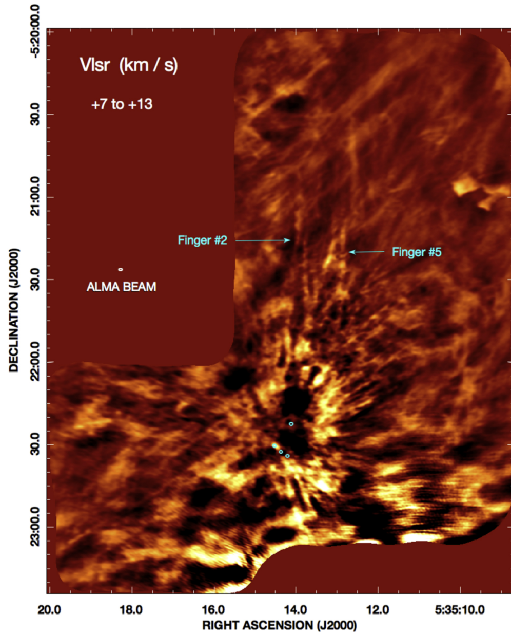
Figure 8. from The ALMA View of the OMC1 Explosion in Orion null 2017 APJ 837 60 doi:10.3847/1538-4357/aa5c8b https://dx.doi.org/10.3847/1538-4357/aa5c8b © 2017. The American Astronomical Society. All rights reserved.
