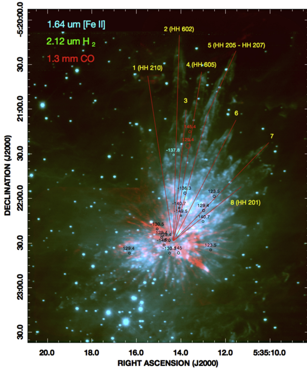
Figure 7. from The ALMA View of the OMC1 Explosion in Orion null 2017 APJ 837 60 doi:10.3847/1538-4357/aa5c8b https://dx.doi.org/10.3847/1538-4357/aa5c8b © 2017. The American Astronomical Society. All rights reserved.
