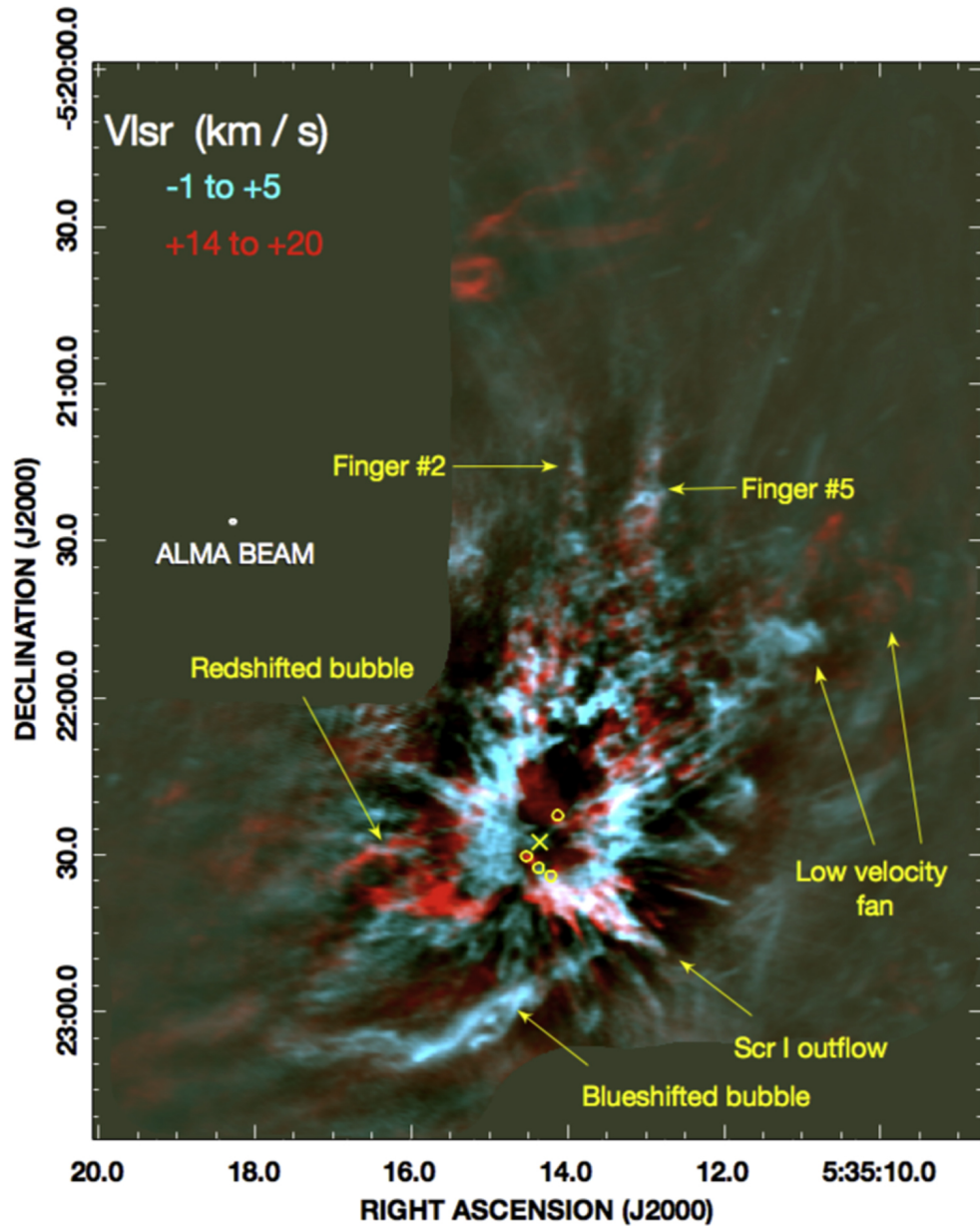
Figure 6. from The ALMA View of the OMC1 Explosion in Orion null 2017 APJ 837 60 doi:10.3847/1538-4357/aa5c8b https://dx.doi.org/10.3847/1538-4357/aa5c8b © 2017. The American Astronomical Society. All rights reserved.
