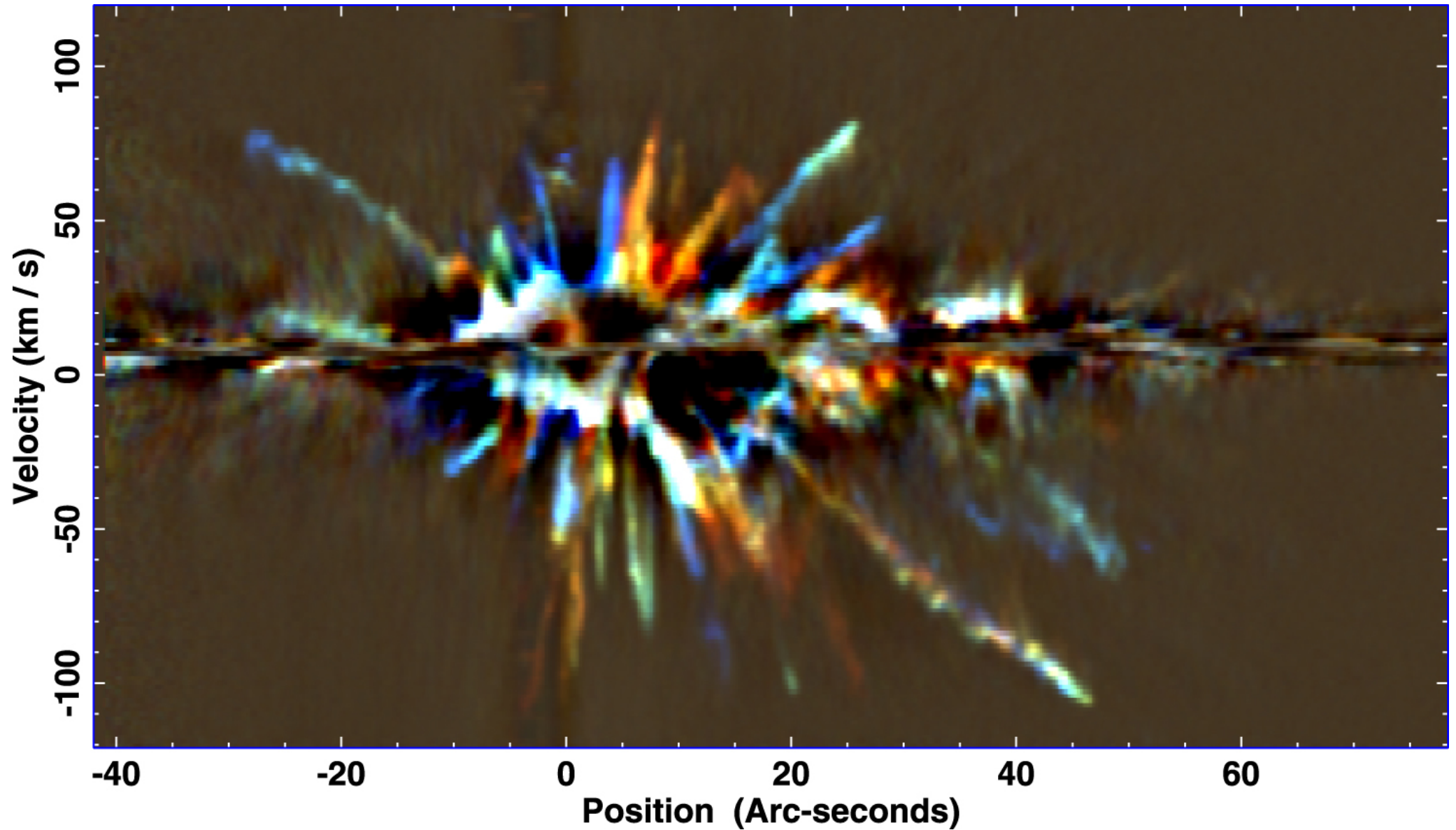
Figure 5. from The ALMA View of the OMC1 Explosion in Orion null 2017 APJ 837 60 doi:10.3847/1538-4357/aa5c8b https://dx.doi.org/10.3847/1538-4357/aa5c8b © 2017. The American Astronomical Society. All rights reserved.
