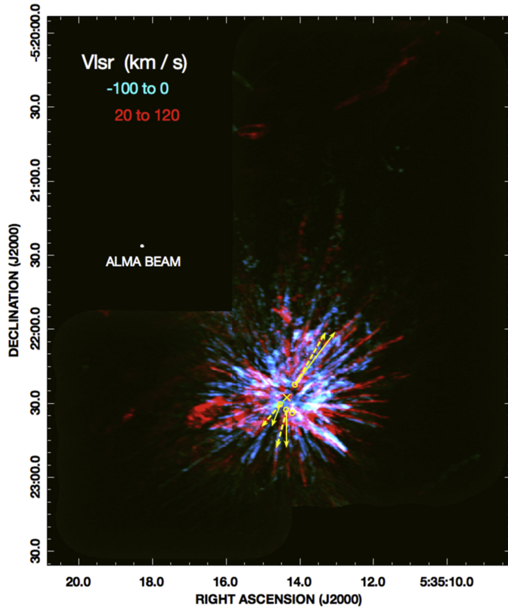
Figure 4. from The ALMA View of the OMC1 Explosion in Orion null 2017 APJ 837 60 doi:10.3847/1538-4357/aa5c8b https://dx.doi.org/10.3847/1538-4357/aa5c8b © 2017. The American Astronomical Society. All rights reserved.
