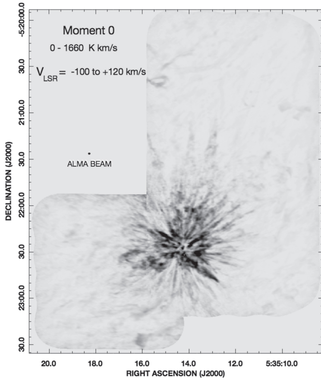
Figure 3. from The ALMA View of the OMC1 Explosion in Orion null 2017 APJ 837 60 doi:10.3847/1538-4357/aa5c8b https://dx.doi.org/10.3847/1538-4357/aa5c8b © 2017. The American Astronomical Society. All rights reserved.
