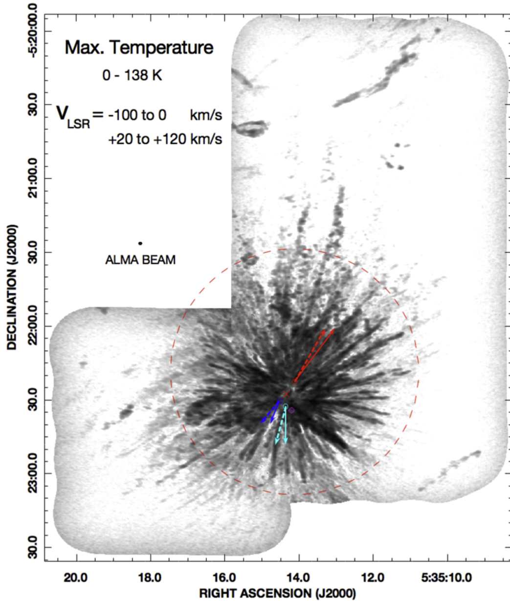
Figure 2. from The ALMA View of the OMC1 Explosion in Orion null 2017 APJ 837 60 doi:10.3847/1538-4357/aa5c8b https://dx.doi.org/10.3847/1538-4357/aa5c8b © 2017. The American Astronomical Society. All rights reserved.
