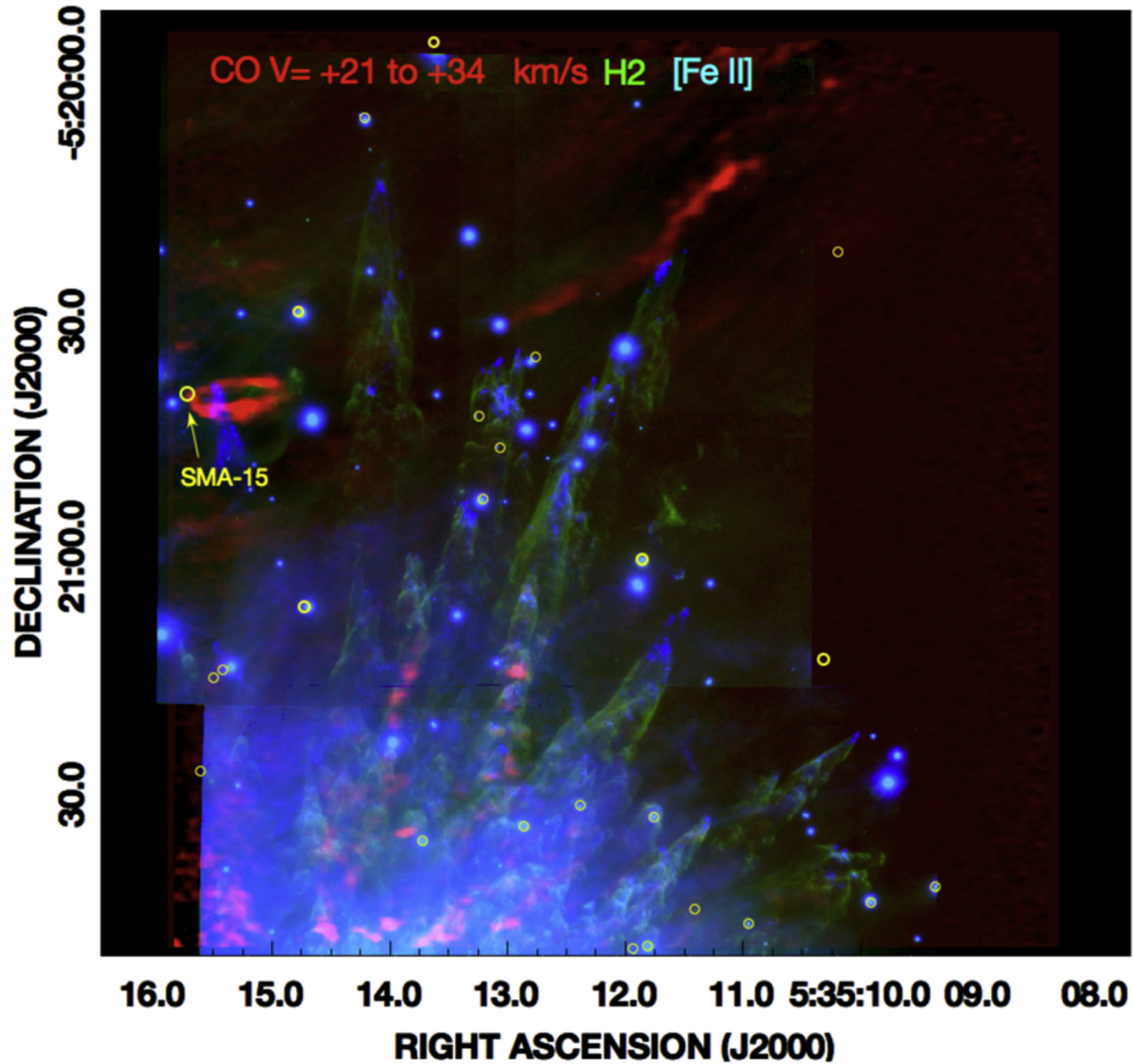
Figure 17. from The ALMA View of the OMC1 Explosion in Orion null 2017 APJ 837 60 doi:10.3847/1538-4357/aa5c8b https://dx.doi.org/10.3847/1538-4357/aa5c8b © 2017. The American Astronomical Society. All rights reserved.
