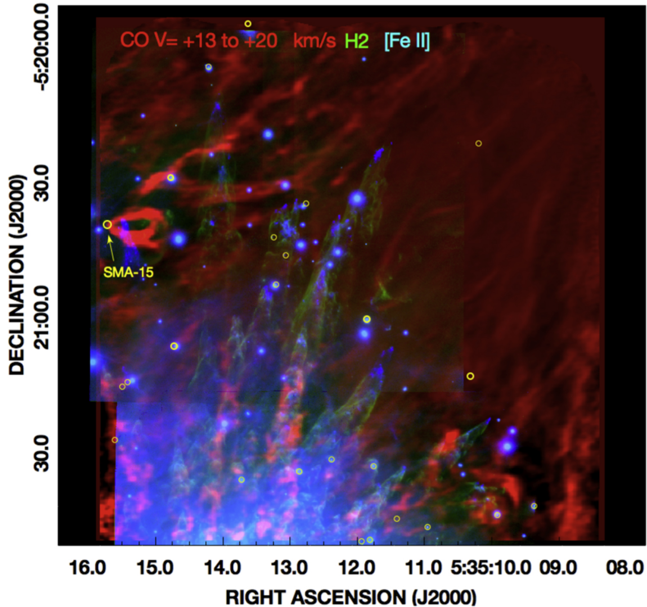
Figure 16. from The ALMA View of the OMC1 Explosion in Orion null 2017 APJ 837 60 doi:10.3847/1538-4357/aa5c8b https://dx.doi.org/10.3847/1538-4357/aa5c8b © 2017. The American Astronomical Society. All rights reserved.
