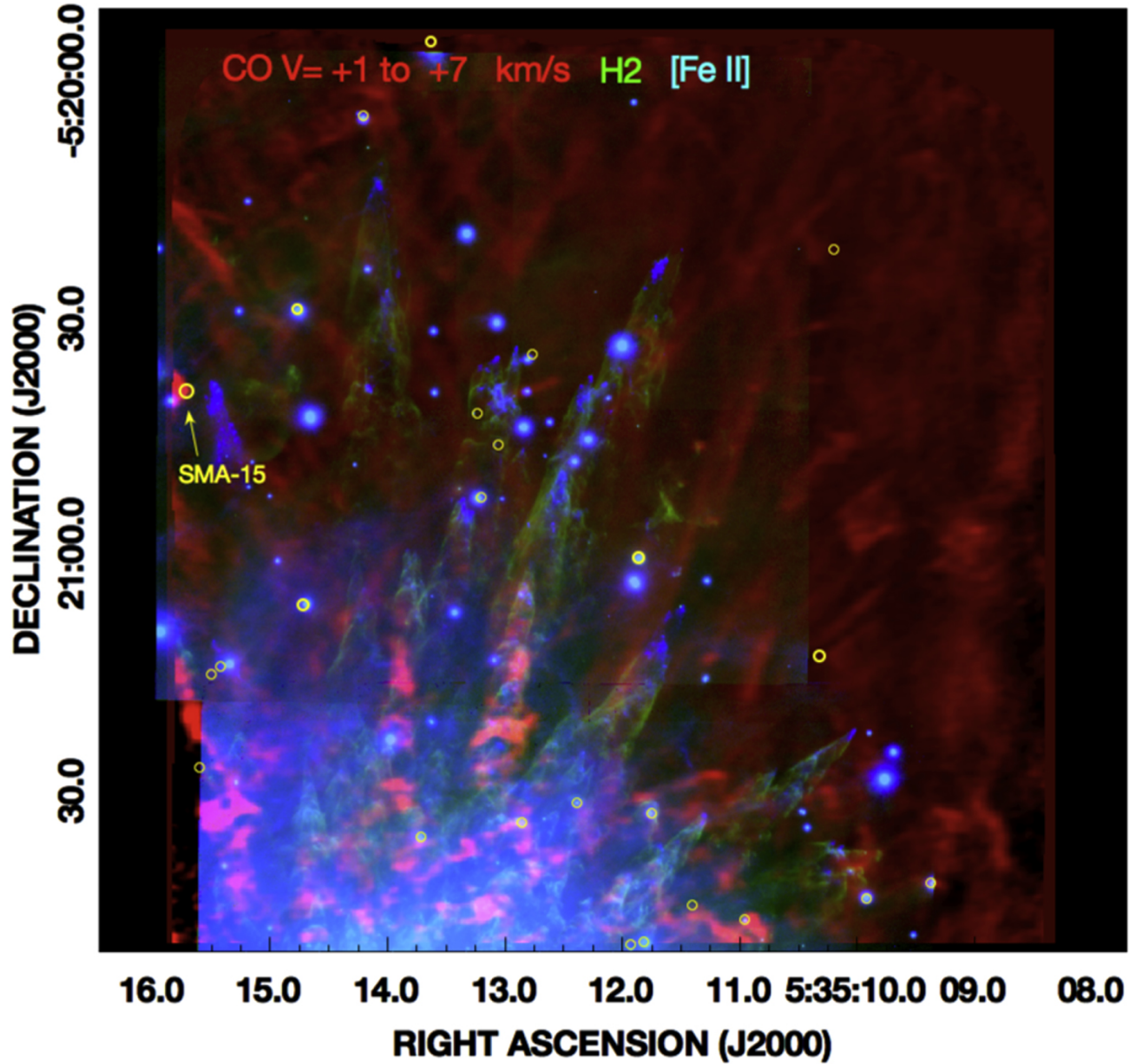
Figure 14. from The ALMA View of the OMC1 Explosion in Orion null 2017 APJ 837 60 doi:10.3847/1538-4357/aa5c8b https://dx.doi.org/10.3847/1538-4357/aa5c8b © 2017. The American Astronomical Society. All rights reserved.
