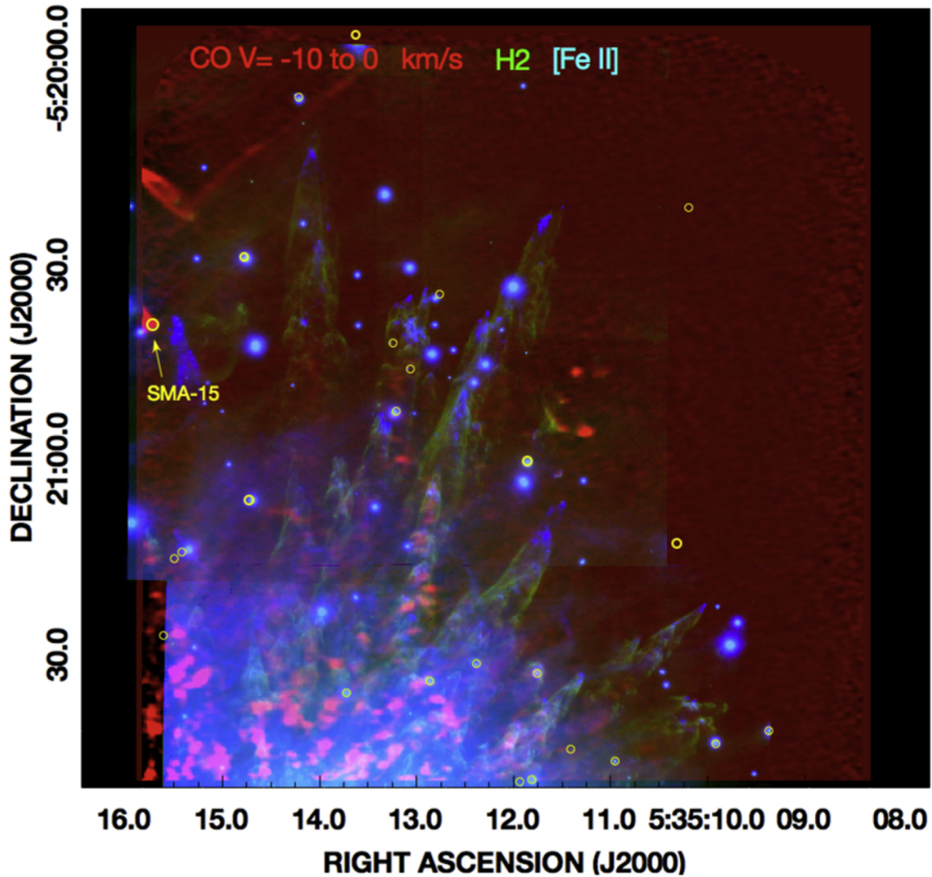
Figure 13. from The ALMA View of the OMC1 Explosion in Orion null 2017 APJ 837 60 doi:10.3847/1538-4357/aa5c8b https://dx.doi.org/10.3847/1538-4357/aa5c8b © 2017. The American Astronomical Society. All rights reserved.
