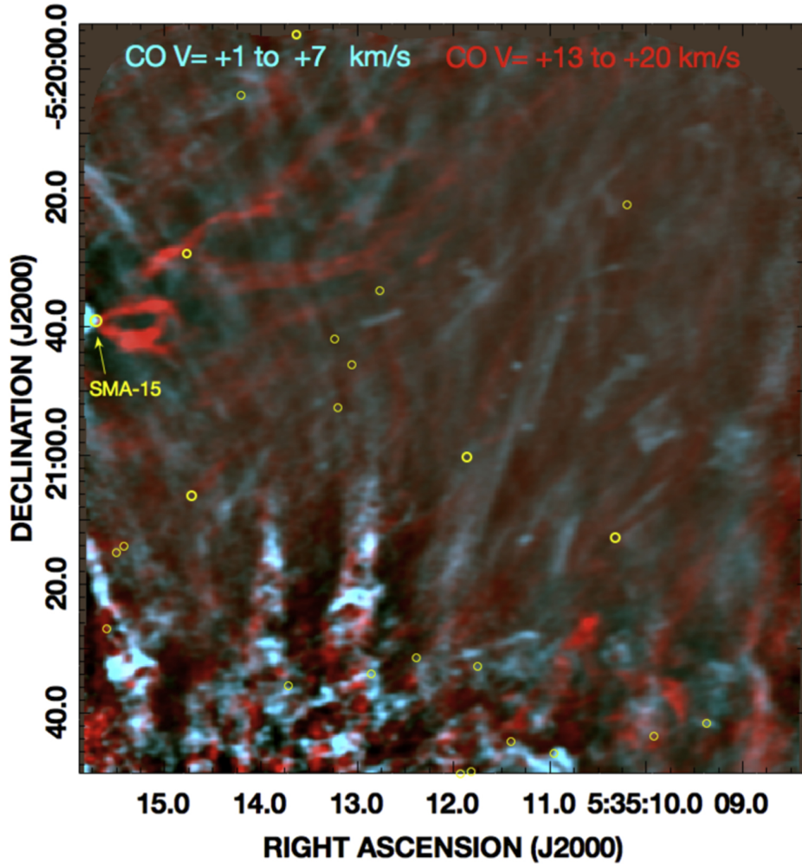
Figure 12. from The ALMA View of the OMC1 Explosion in Orion null 2017 APJ 837 60 doi:10.3847/1538-4357/aa5c8b https://dx.doi.org/10.3847/1538-4357/aa5c8b © 2017. The American Astronomical Society. All rights reserved.
