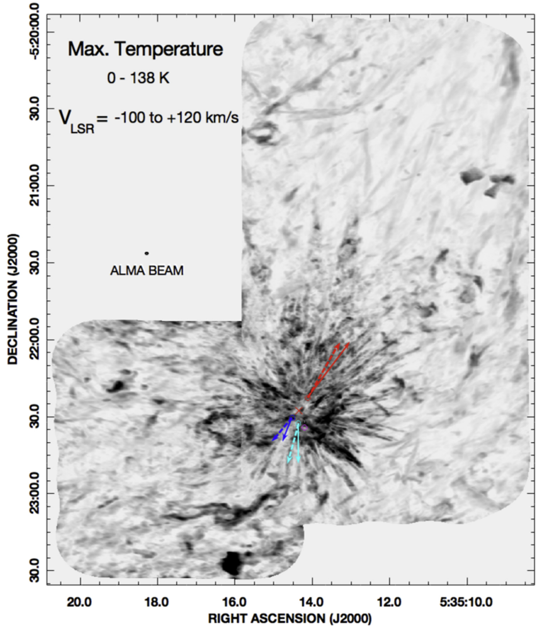
Figure 1. from The ALMA View of the OMC1 Explosion in Orion null 2017 APJ 837 60 doi:10.3847/1538-4357/aa5c8b https://dx.doi.org/10.3847/1538-4357/aa5c8b © 2017. The American Astronomical Society. All rights reserved.
