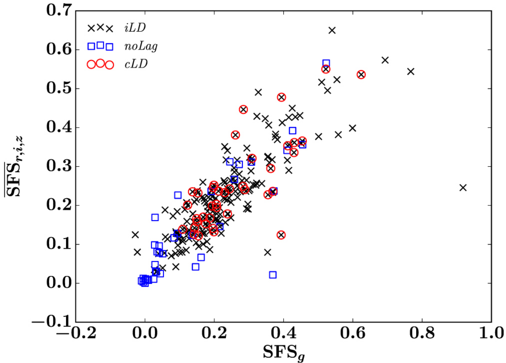
Figure 9. from Detection of Time Lags between Quasar Continuum Emission Bands Based On Pan-STARRS Light Curves null 2017 APJ 836 186 doi:10.3847/1538-4357/aa5b91 https://dx.doi.org/10.3847/1538-4357/aa5b91 © 2017. The American Astronomical Society. All rights reserved.
