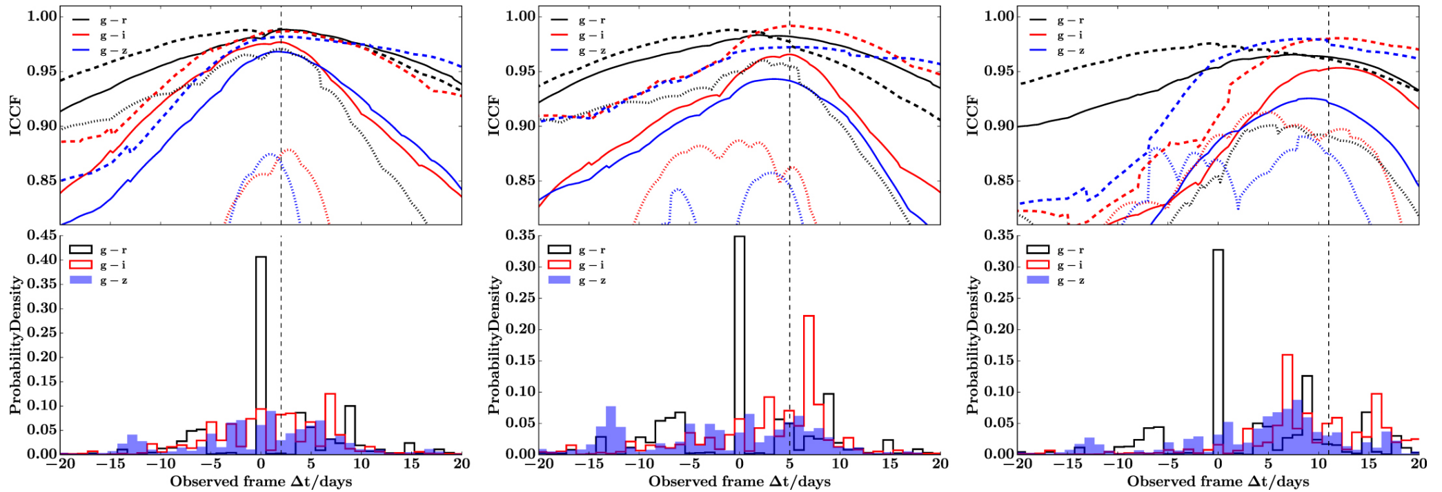
Figure 7. from Detection of Time Lags between Quasar Continuum Emission Bands Based On Pan-STARRS Light Curves null 2017 APJ 836 186 doi:10.3847/1538-4357/aa5b91 https://dx.doi.org/10.3847/1538-4357/aa5b91
