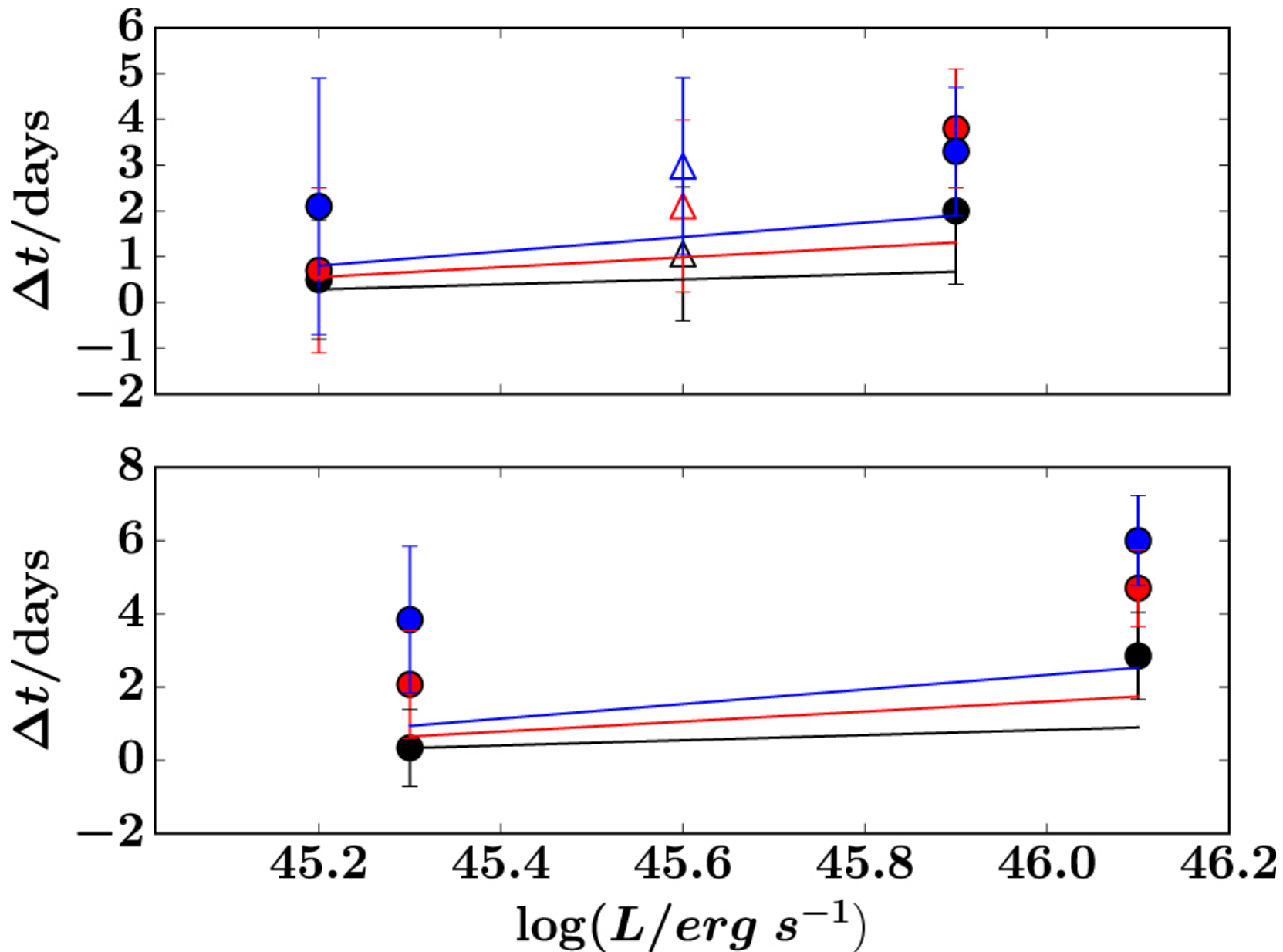
Figure 17. from Detection of Time Lags between Quasar Continuum Emission Bands Based On Pan-STARRS Light Curves null 2017 APJ 836 186 doi:10.3847/1538-4357/aa5b91 https://dx.doi.org/10.3847/1538-4357/aa5b91 © 2017. The American Astronomical Society. All rights reserved.
