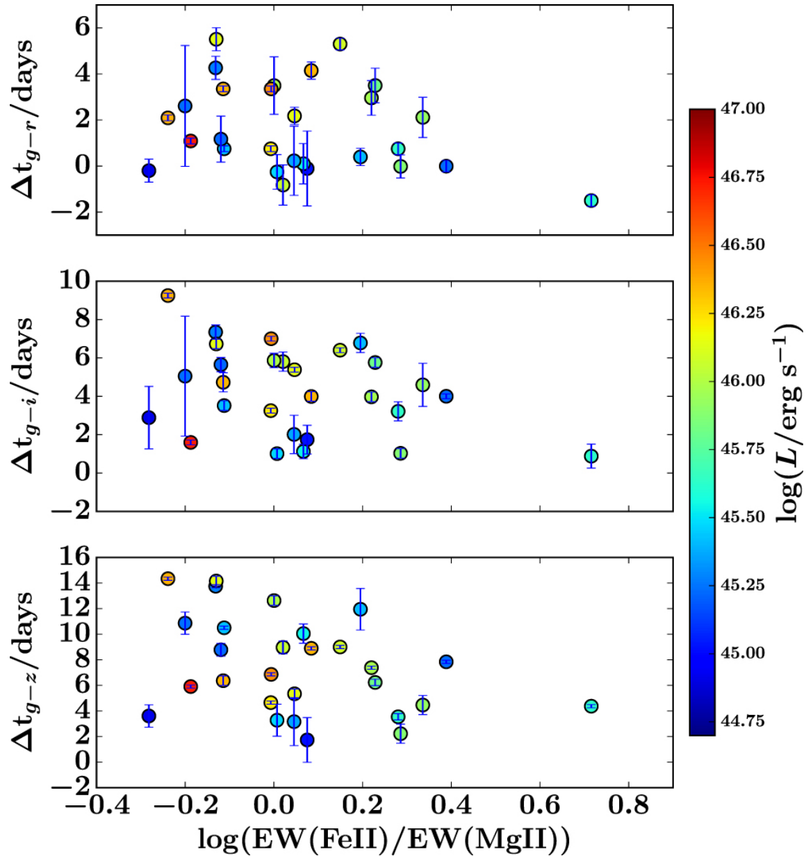
Figure 16. from Detection of Time Lags between Quasar Continuum Emission Bands Based On Pan-STARRS Light Curves null 2017 APJ 836 186 doi:10.3847/1538-4357/aa5b91 https://dx.doi.org/10.3847/1538-4357/aa5b91 © 2017. The American Astronomical Society. All rights reserved.
