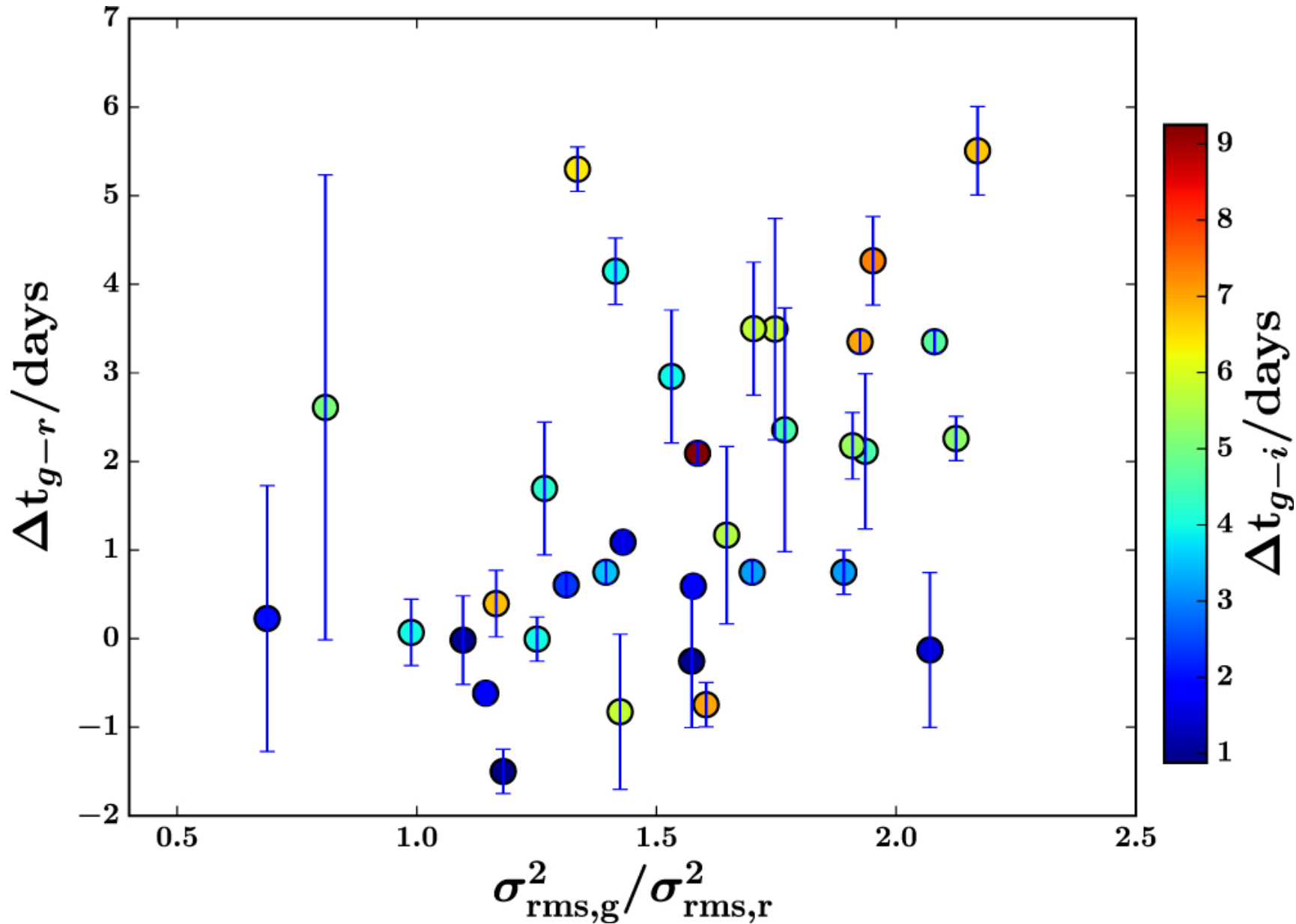
Figure 15. from Detection of Time Lags between Quasar Continuum Emission Bands Based On Pan-STARRS Light Curves null 2017 APJ 836 186 doi:10.3847/1538-4357/aa5b91 https://dx.doi.org/10.3847/1538-4357/aa5b91 © 2017. The American Astronomical Society. All rights reserved.
