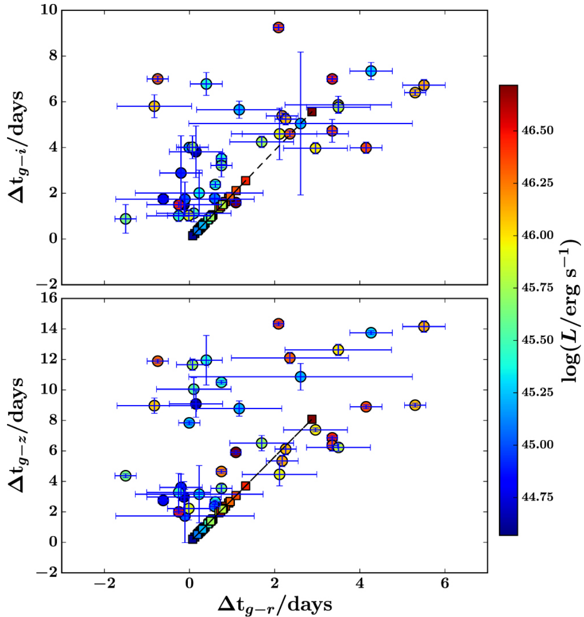
Figure 14. from Detection of Time Lags between Quasar Continuum Emission Bands Based On Pan-STARRS Light Curves null 2017 APJ 836 186 doi:10.3847/1538-4357/aa5b91 https://dx.doi.org/10.3847/1538-4357/aa5b91
