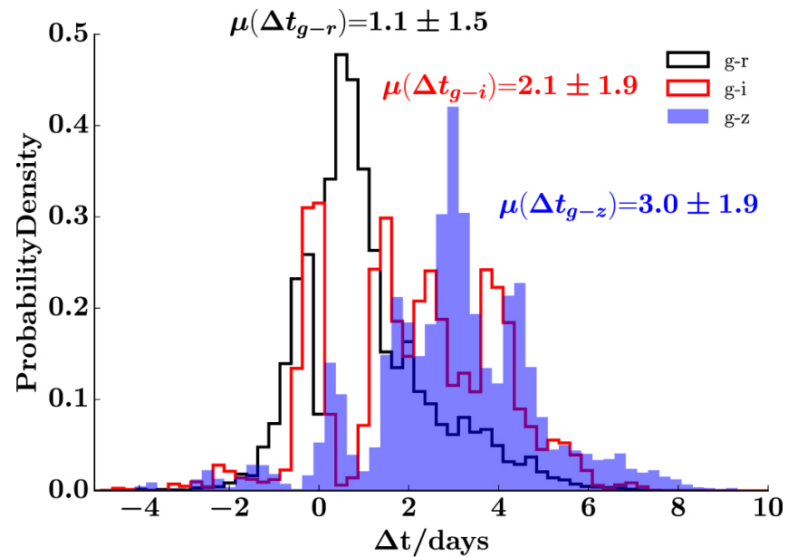
Figure 10. from Detection of Time Lags between Quasar Continuum Emission Bands Based On Pan-STARRS Light Curves null 2017 APJ 836 186 doi:10.3847/1538-4357/aa5b91 https://dx.doi.org/10.3847/1538-4357/aa5b91
