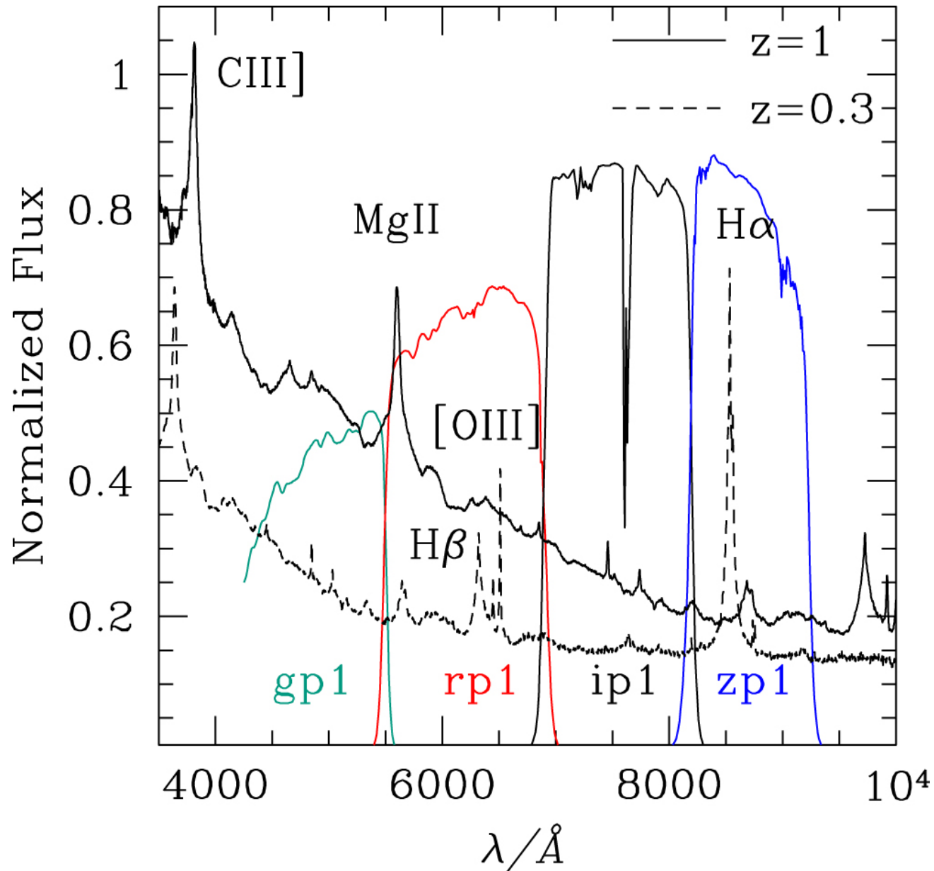
Figure 1. from Detection of Time Lags between Quasar Continuum Emission Bands Based On Pan-STARRS Light Curves null 2017 APJ 836 186 doi:10.3847/1538-4357/aa5b91 https://dx.doi.org/10.3847/1538-4357/aa5b91 © 2017. The American Astronomical Society. All rights reserved.
