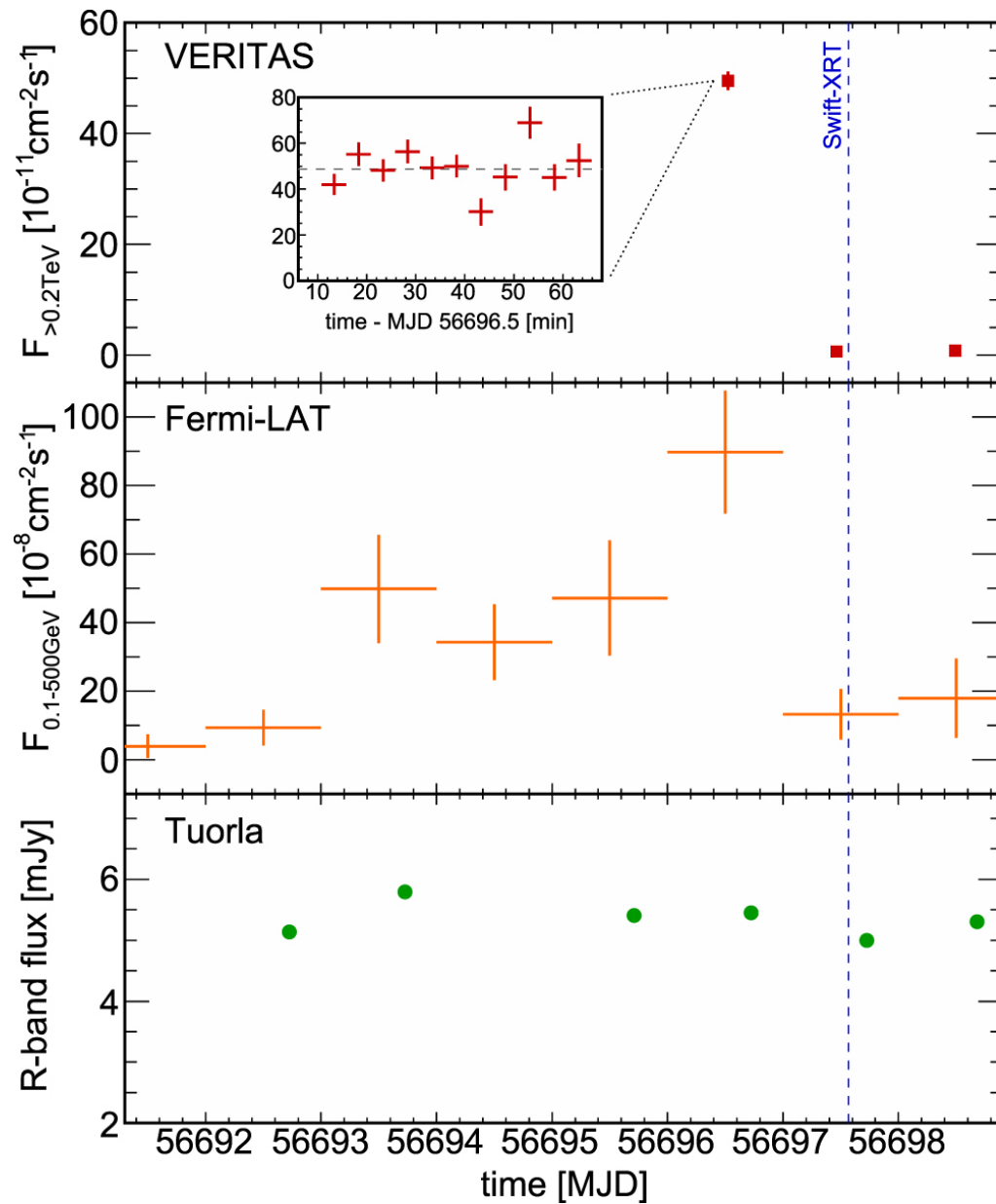
Figure 3. from A Luminous and Isolated Gamma-Ray Flare from the Blazar B2 1215+30 null 2017 APJ 836 205 doi:10.3847/1538-4357/836/2/205 https://dx.doi.org/10.3847/1538-4357/836/2/205 © 2017. The American Astronomical Society. All rights reserved.
