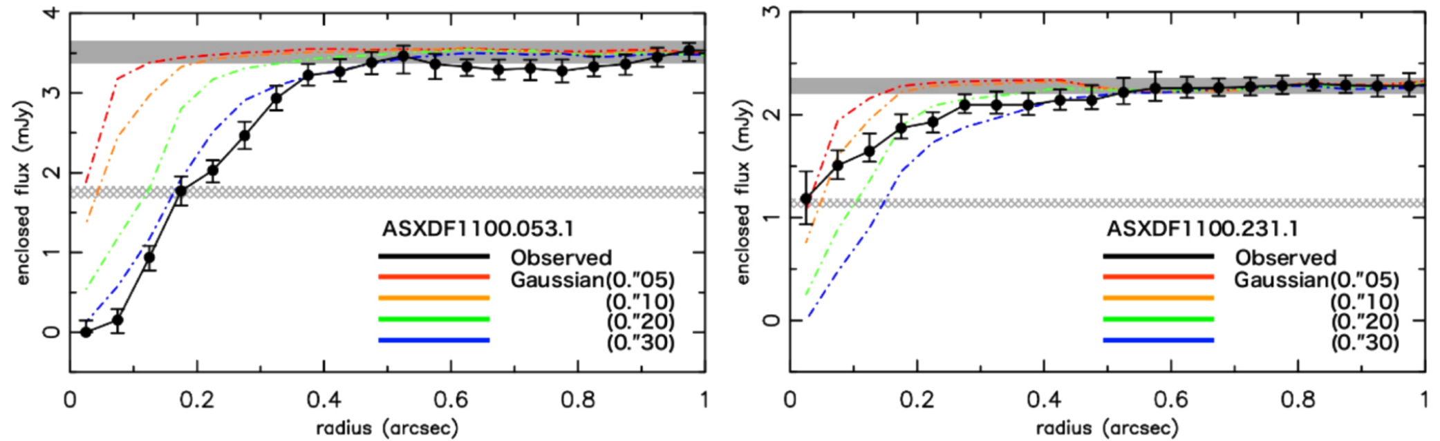
Figure 9. from Extremely Red Submillimeter Galaxies: New z = 4-6 Candidates Discovered Using ALMA and Jansky VLA null 2017 APJ 835 286 doi:10.3847/1538-4357/835/2/286 https://dx.doi.org/10.3847/1538-4357/835/2/286 © 2017. The American Astronomical Society. All rights reserved.
