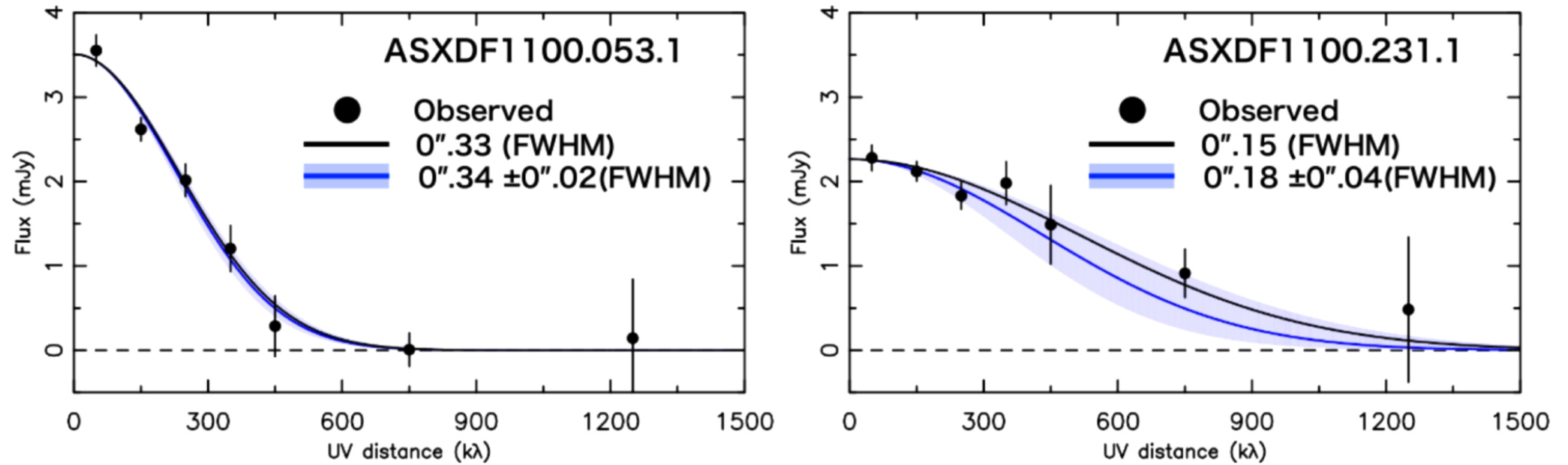
Figure 8. from Extremely Red Submillimeter Galaxies: New z = 4-6 Candidates Discovered Using ALMA and Jansky VLA null 2017 APJ 835 286 doi:10.3847/1538-4357/835/2/286 https://dx.doi.org/10.3847/1538-4357/835/2/286 © 2017. The American Astronomical Society. All rights reserved.
