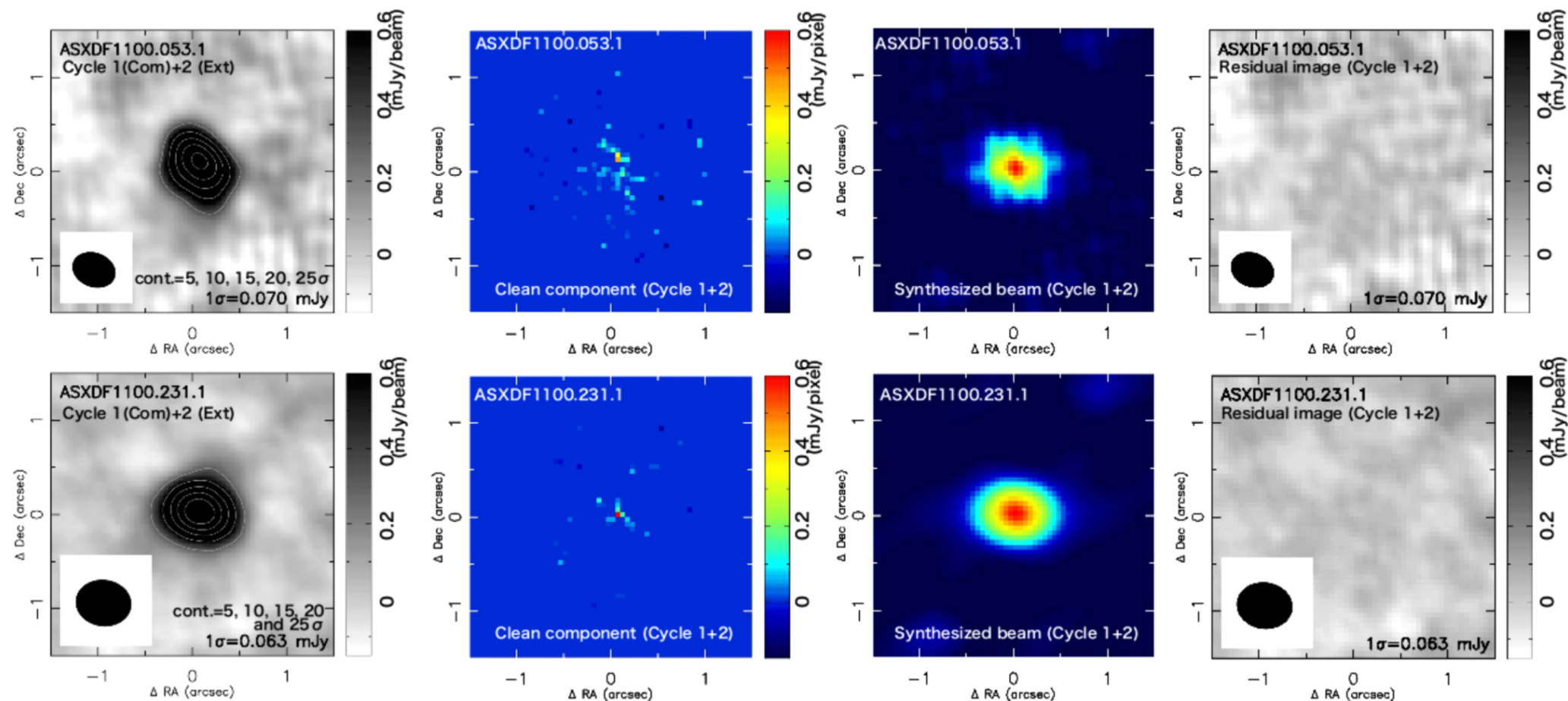
Figure 7. from Extremely Red Submillimeter Galaxies: New z = 4-6 Candidates Discovered Using ALMA and Jansky VLA null 2017 APJ 835 286 doi:10.3847/1538-4357/835/2/286 https://dx.doi.org/10.3847/1538-4357/835/2/286 © 2017. The American Astronomical Society. All rights reserved.
