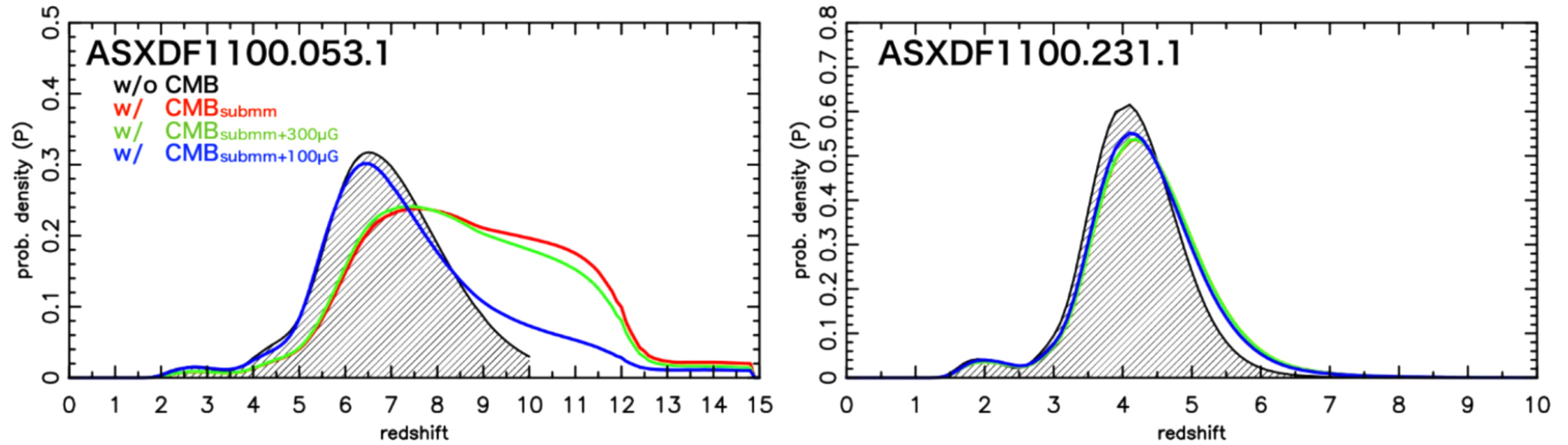
Figure 6. from Extremely Red Submillimeter Galaxies: New z \sim 4-6 Candidates Discovered Using ALMA and Jansky VLA null 2017 APJ 835 286 doi:10.3847/1538-4357/835/2/286 https://dx.doi.org/10.3847/1538-4357/835/2/286 © 2017. The American Astronomical Society. All rights reserved.
