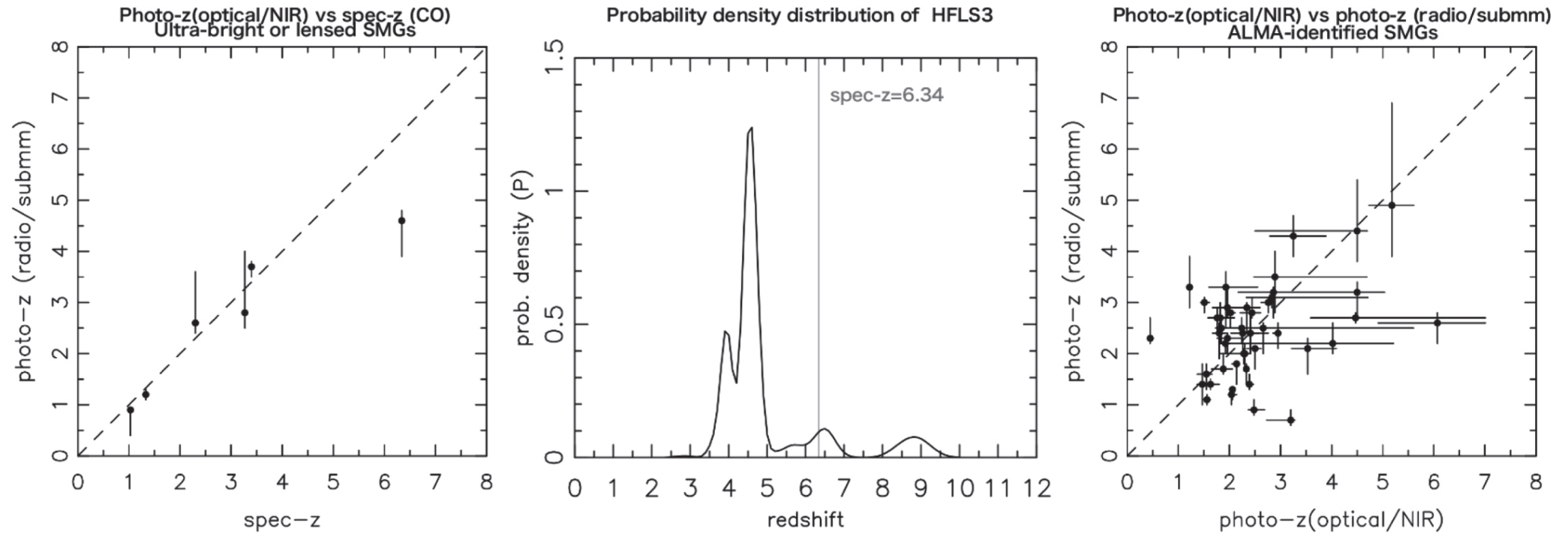
Figure 5. from Extremely Red Submillimeter Galaxies: New z = 4\text{--}6 Candidates Discovered Using ALMA and Jansky VLA null 2017 APJ 835 286 doi:10.3847/1538-4357/835/2/286 https://dx.doi.org/10.3847/1538-4357/835/2/286
