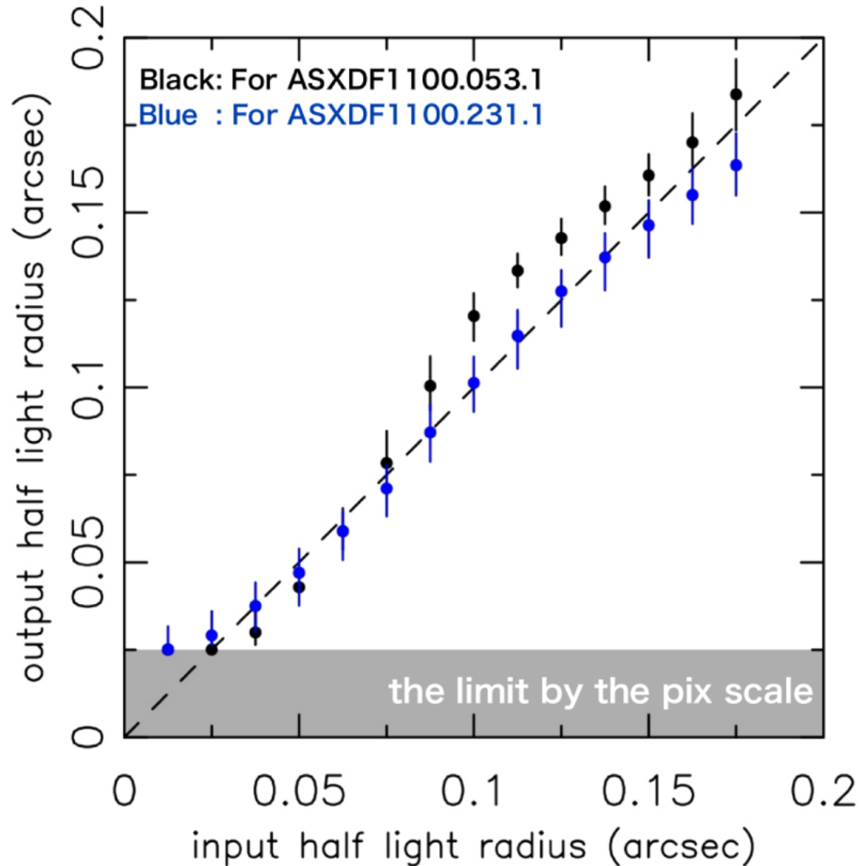
Figure 14. from Extremely Red Submillimeter Galaxies: New z = 4-6 Candidates Discovered Using ALMA and Jansky VLA null 2017 APJ 835 286 doi:10.3847/1538-4357/835/2/286 https://dx.doi.org/10.3847/1538-4357/835/2/286 © 2017. The American Astronomical Society. All rights reserved.
