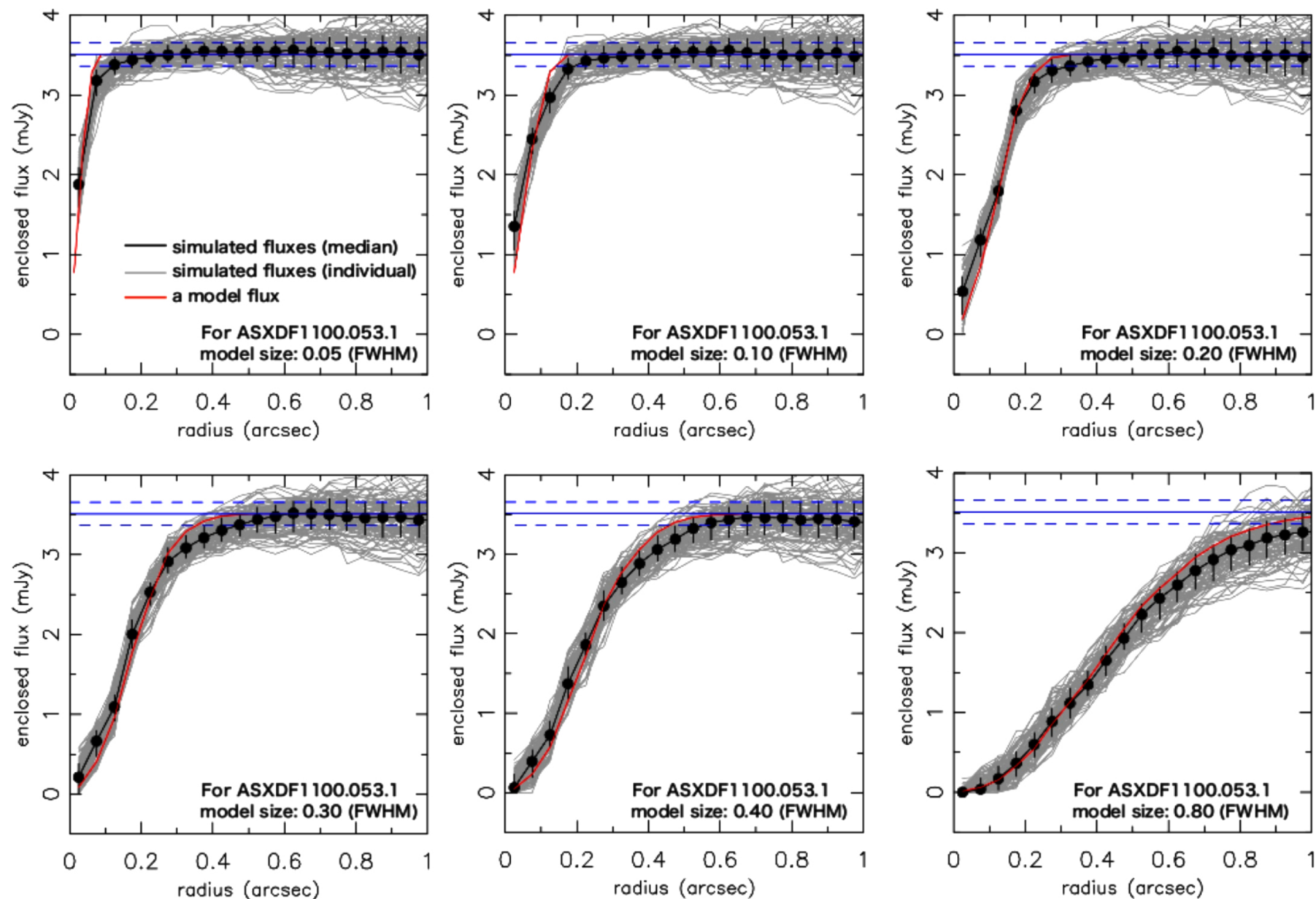
Figure 13. from Extremely Red Submillimeter Galaxies: New z 4–6 Candidates Discovered Using ALMA and Jansky VLA null 2017 APJ 835 286 doi:10.3847/1538-4357/835/2/286 https://dx.doi.org/10.3847/1538-4357/835/2/286
