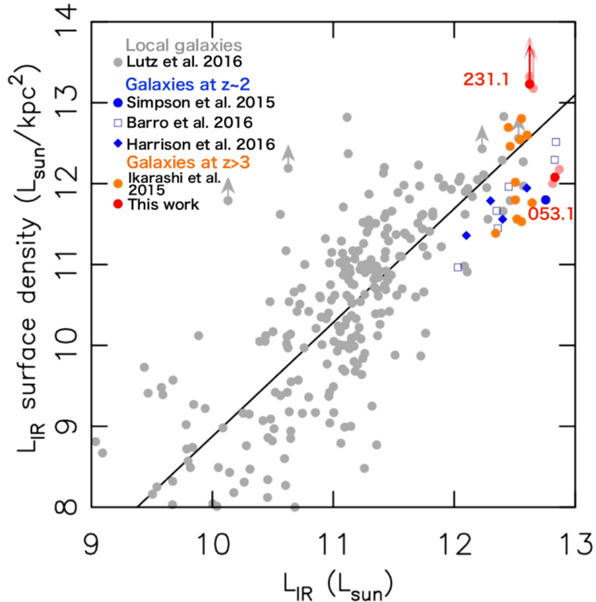
Figure 12. from Extremely Red Submillimeter Galaxies: New z = 4-6 Candidates Discovered Using ALMA and Jansky VLA null 2017 APJ 835 286 doi:10.3847/1538-4357/835/2/286 https://dx.doi.org/10.3847/1538-4357/835/2/286 © 2017. The American Astronomical Society. All rights reserved.
