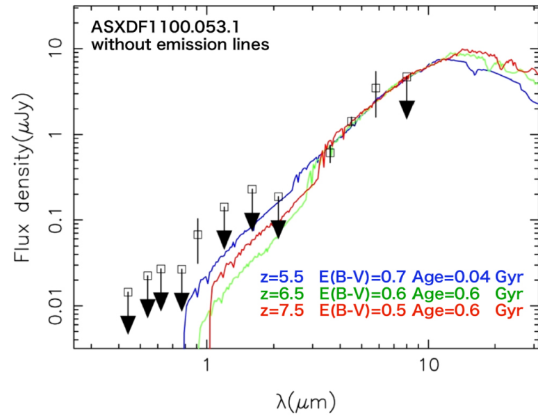
Figure 10. from Extremely Red Submillimeter Galaxies: New z 4–6 Candidates Discovered Using ALMA and Jansky VLA null 2017 APJ 835 286 doi:10.3847/1538-4357/835/2/286 https://dx.doi.org/10.3847/1538-4357/835/2/286 © 2017. The American Astronomical Society. All rights reserved.
