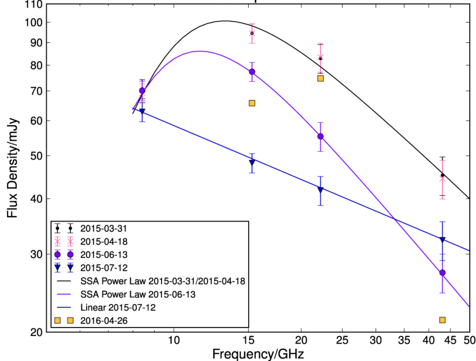
Figure 5. from The Relativistic Jet-accretion Flow–wind Connection in Mrk 231 null 2017 APJ 836 155 doi:10.3847/1538-4357/836/2/155 https://dx.doi.org/10.3847/1538-4357/836/2/155 © 2017. The American Astronomical Society. All rights reserved.
