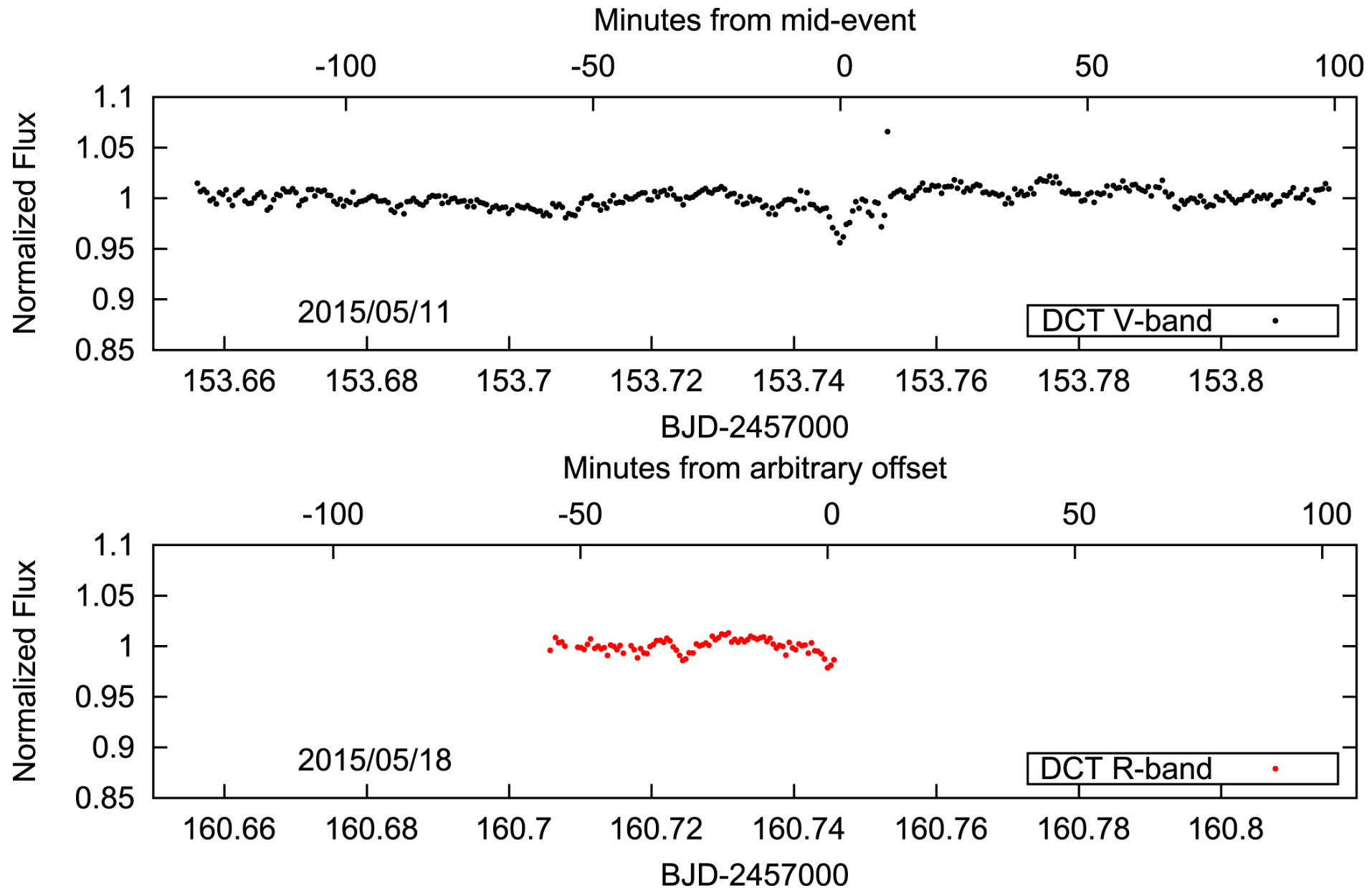
Figure 9. from Multiwavelength Transit Observations of the Candidate Disintegrating Planetesimals Orbiting WD 1145+017 null 2017 APJ 836 82 doi:10.3847/1538-4357/836/1/82 https://dx.doi.org/10.3847/1538-4357/836/1/82 © 2017. The American Astronomical Society. All rights reserved.
