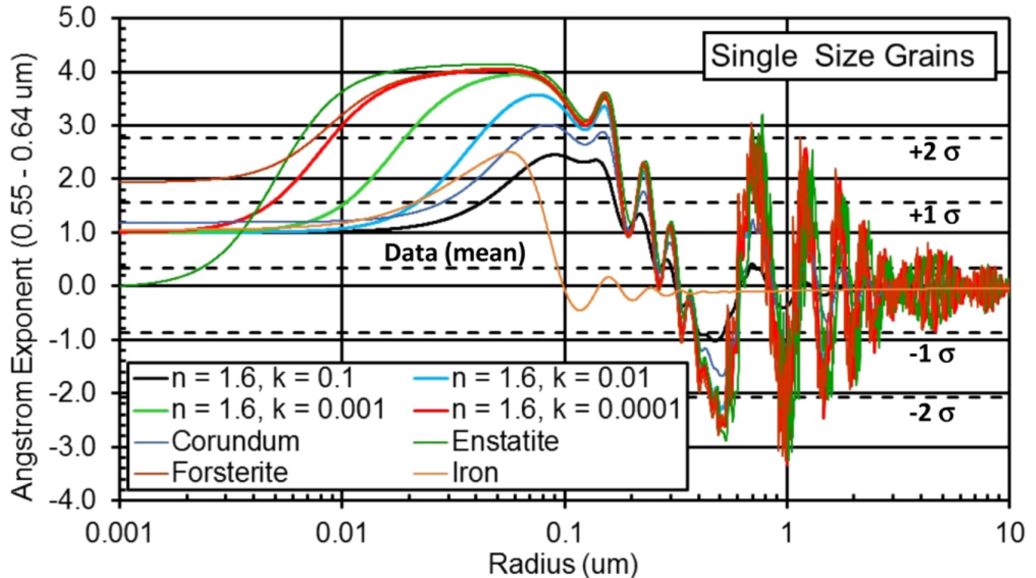
Figure 8. from Multiwavelength Transit Observations of the Candidate Disintegrating Planetesimals Orbiting WD 1145+017 null 2017 APJ 836 82 doi:10.3847/1538-4357/836/1/82 https://dx.doi.org/10.3847/1538-4357/836/1/82 © 2017. The American Astronomical Society. All rights reserved.
