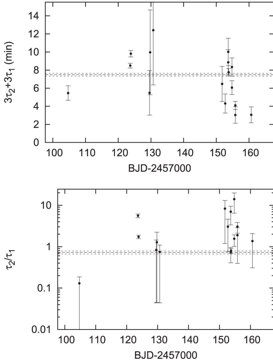
Figure 7. from Multiwavelength Transit Observations of the Candidate Disintegrating Planetesimals Orbiting WD 1145+017 null 2017 APJ 836 82 doi:10.3847/1538-4357/836/1/82 https://dx.doi.org/10.3847/1538-4357/836/1/82 © 2017. The American Astronomical Society. All rights reserved.
