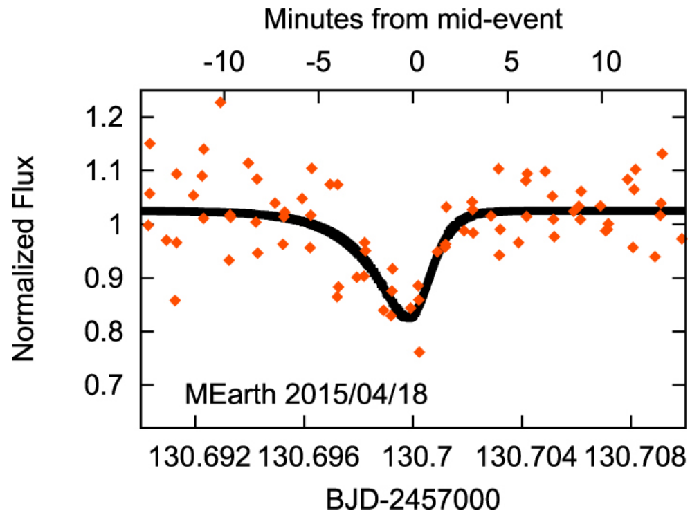
Figure 6. from Multiwavelength Transit Observations of the Candidate Disintegrating Planetesimals Orbiting WD 1145+017 null 2017 APJ 836 82 doi:10.3847/1538-4357/836/1/82 https://dx.doi.org/10.3847/1538-4357/836/1/82
