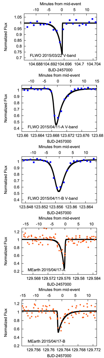
Figure 5. from Multiwavelength Transit Observations of the Candidate Disintegrating Planetesimals Orbiting WD 1145+017 null 2017 APJ 836 82 doi:10.3847/1538-4357/836/1/82 https://dx.doi.org/10.3847/1538-4357/836/1/82 © 2017. The American Astronomical Society. All rights reserved.
