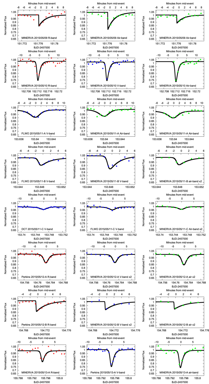
Figure 4. from Multiwavelength Transit Observations of the Candidate Disintegrating Planetesimals Orbiting WD 1145+017 null 2017 APJ 836 82 doi:10.3847/1538-4357/836/1/82 https://dx.doi.org/10.3847/1538-4357/836/1/82 © 2017. The American Astronomical Society. All rights reserved.
