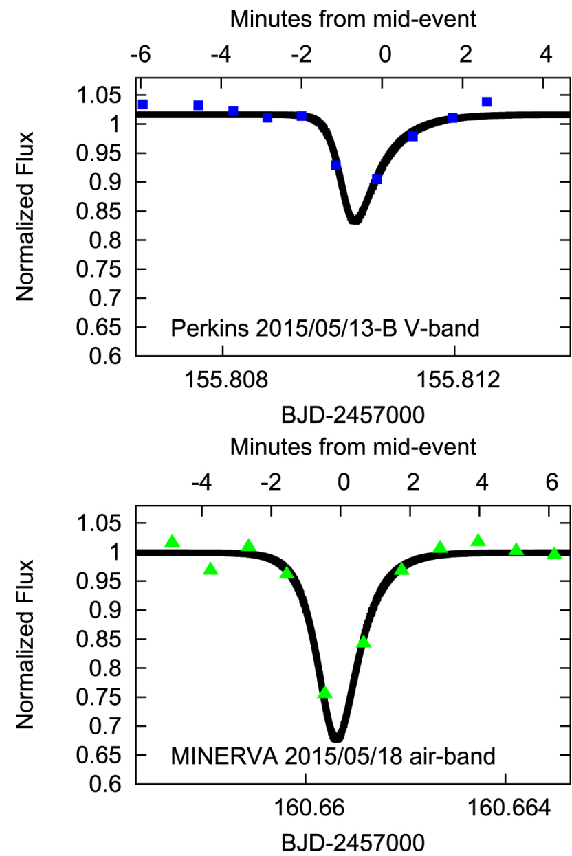
Figure 3. from Multiwavelength Transit Observations of the Candidate Disintegrating Planetesimals Orbiting WD 1145+017 null 2017 APJ 836 82 doi:10.3847/1538-4357/836/1/82 https://dx.doi.org/10.3847/1538-4357/836/1/82 © 2017. The American Astronomical Society. All rights reserved.
