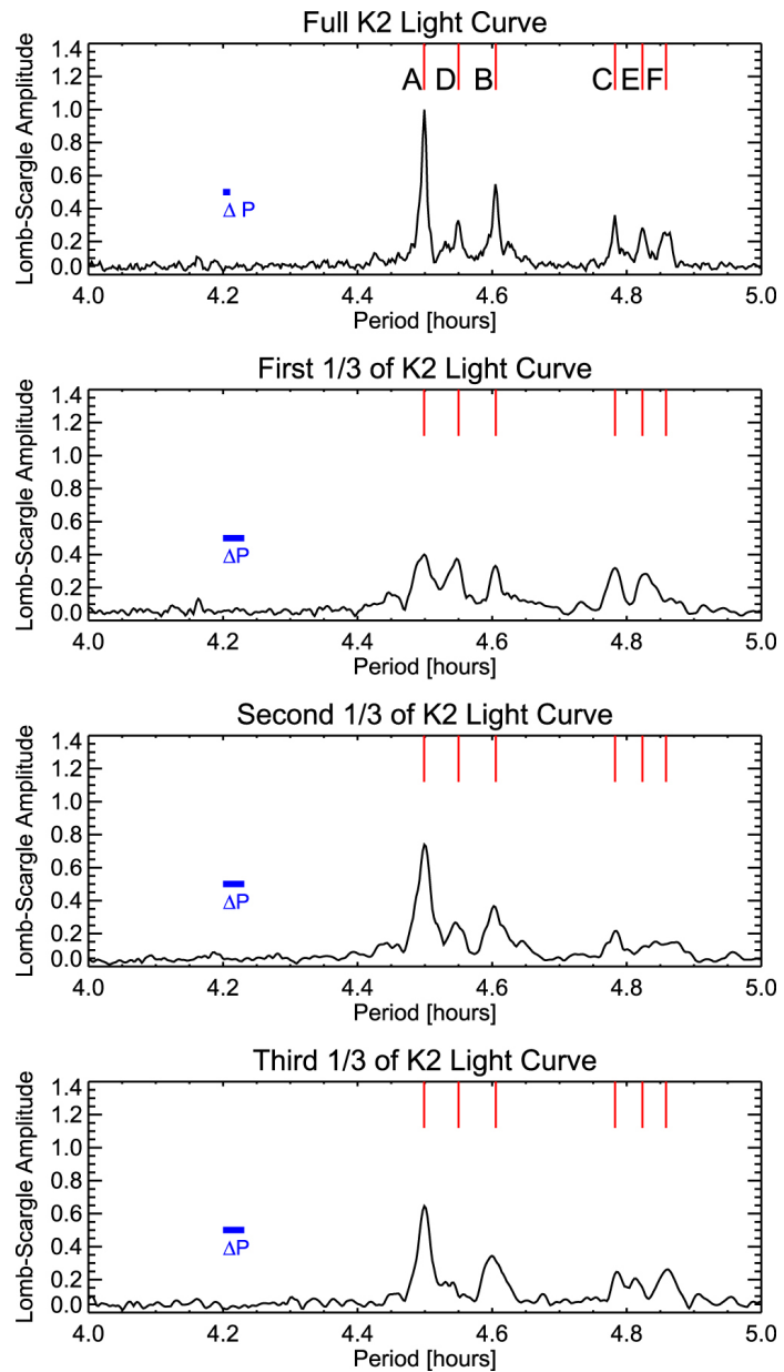
Figure 11. from Multiwavelength Transit Observations of the Candidate Disintegrating Planetesimals Orbiting WD 1145+017 null 2017 APJ 836 82 doi:10.3847/1538-4357/836/1/82 https://dx.doi.org/10.3847/1538-4357/836/1/82
