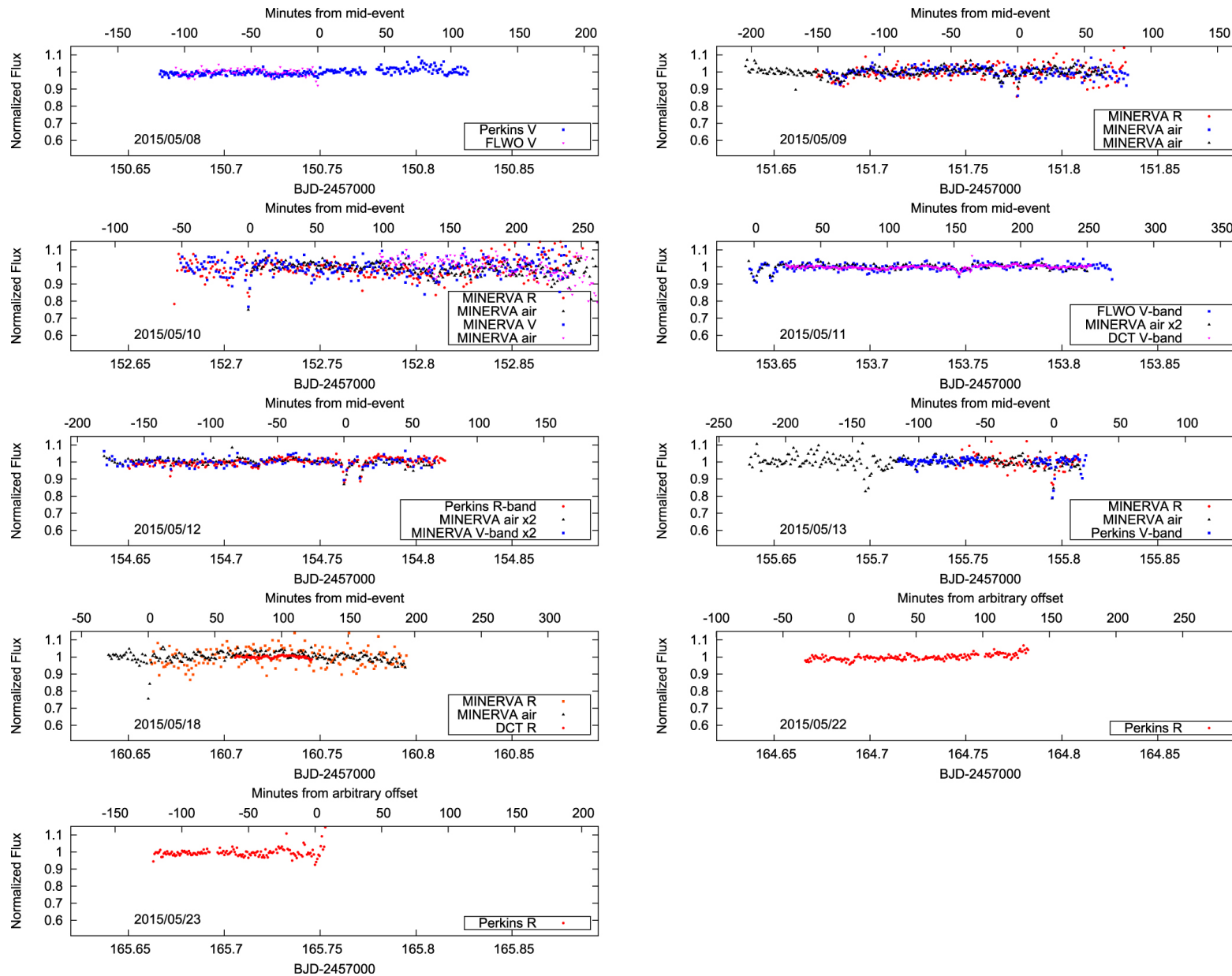
Figure 1. from Multiwavelength Transit Observations of the Candidate Disintegrating Planetesimals Orbiting WD 1145+017 null 2017 APJ 836 82 doi:10.3847/1538-4357/836/1/82 https://dx.doi.org/10.3847/1538-4357/836/1/82 © 2017. The American Astronomical Society. All rights reserved.
