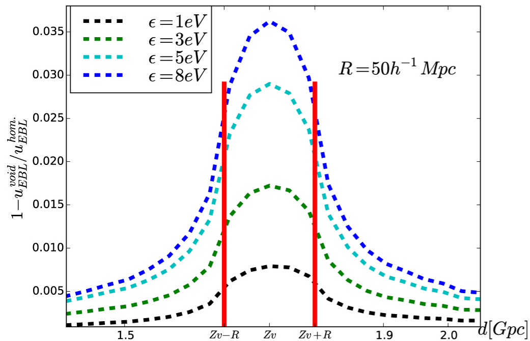
Figure 4. from EBL Inhomogeneity and Hard-Spectrum Gamma-Ray Sources null 2017 APJ 835 237 doi:10.3847/1538-4357/835/2/237 https://dx.doi.org/10.3847/1538-4357/835/2/237 © 2017. The American Astronomical Society. All rights reserved.
