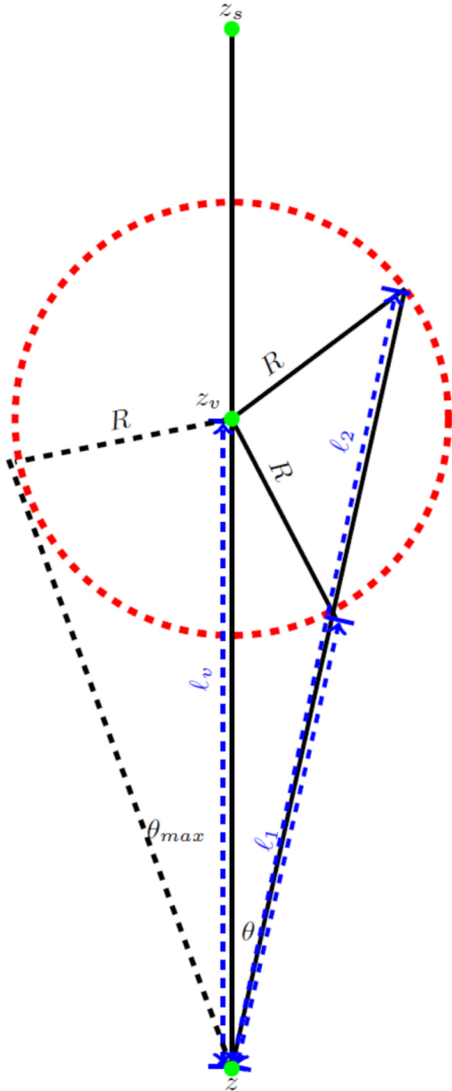
Figure 1. from EBL Inhomogeneity and Hard-Spectrum Gamma-Ray Sources null 2017 APJ 835 237 doi:10.3847/1538-4357/835/2/237 https://dx.doi.org/10.3847/1538-4357/835/2/237 © 2017. The American Astronomical Society. All rights reserved.
