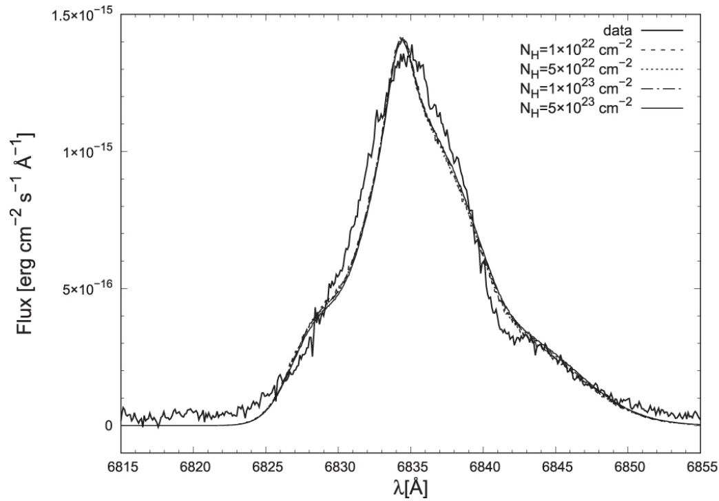
Figure 5. from A PROFILE ANALYSIS OF RAMAN-SCATTERED O VI BANDS AT 6825 AND 7082 IN SANDULEAK'S STAR null 2016 APJ 833 286 doi:10.3847/1538-4357/833/2/286 https://dx.doi.org/10.3847/1538-4357/833/2/286 © 2016. The American Astronomical Society. All rights reserved.
