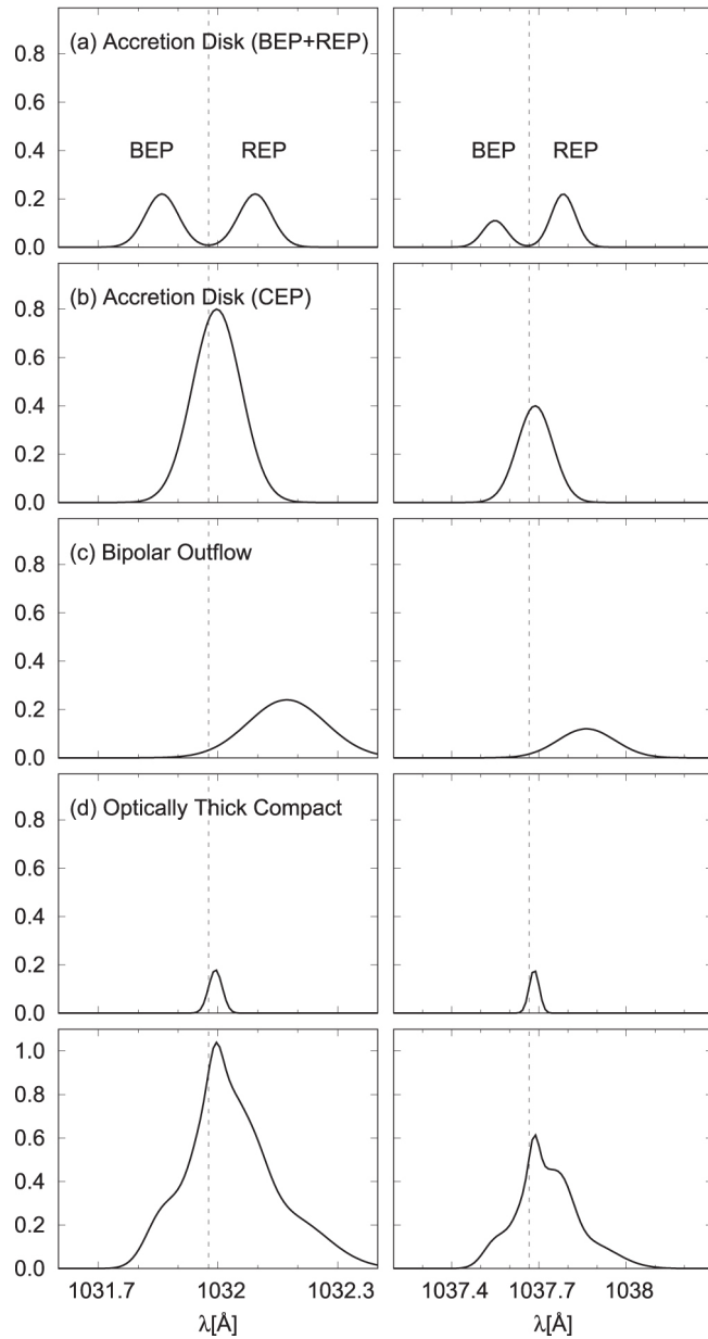
Figure 4. from A PROFILE ANALYSIS OF RAMAN-SCATTERED O VI BANDS AT 6825 AND 7082 IN SANDULEAK'S STAR null 2016 APJ 833 286 doi:10.3847/1538-4357/833/2/286 https://dx.doi.org/10.3847/1538-4357/833/2/286 © 2016. The American Astronomical Society. All rights reserved.
