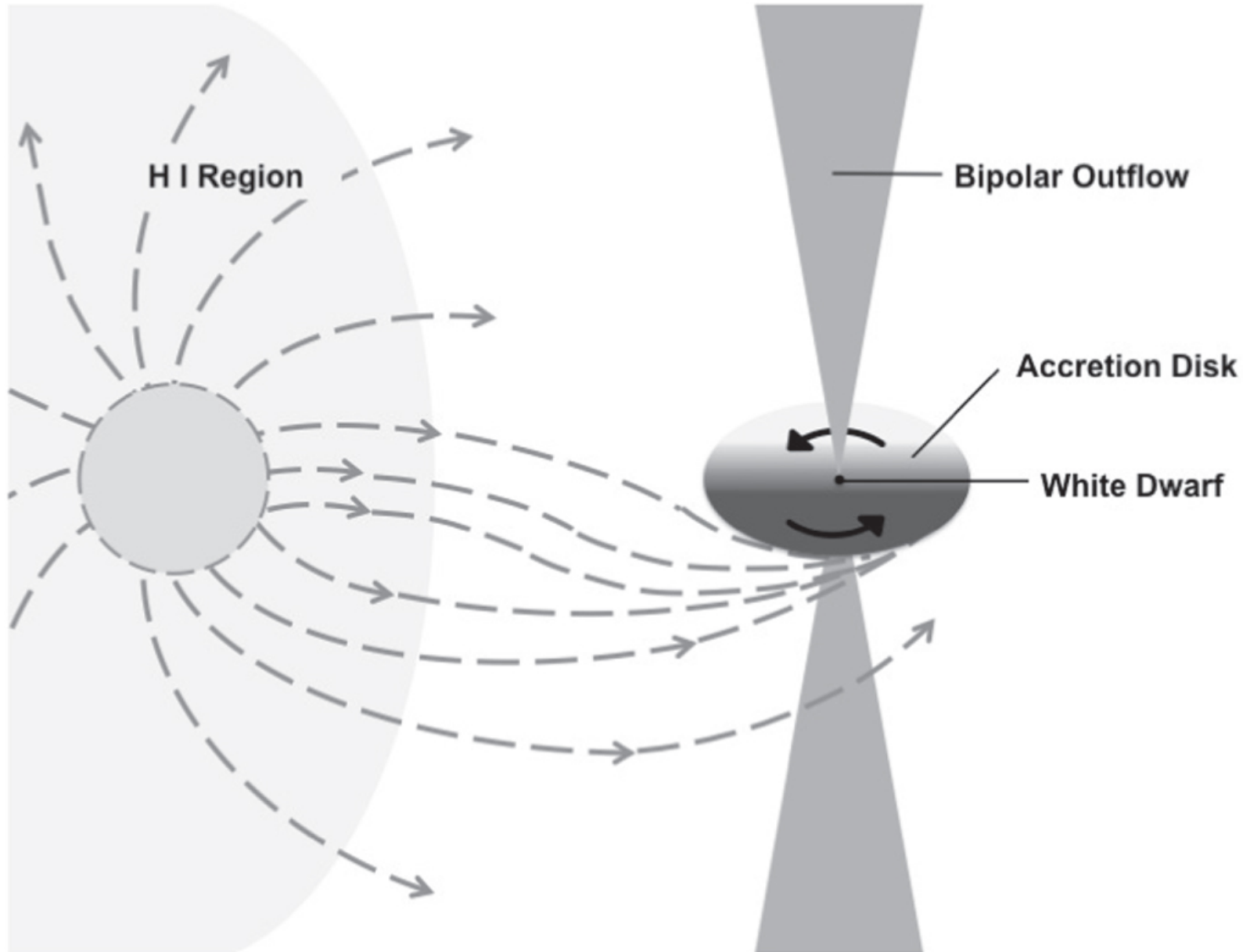
Figure 3. from A PROFILE ANALYSIS OF RAMAN-SCATTERED O VI BANDS AT 6825 AND 7082 IN SANDULEAK'S STAR null 2016 APJ 833 286 doi:10.3847/1538-4357/833/2/286 https://dx.doi.org/10.3847/1538-4357/833/2/286 © 2016. The American Astronomical Society. All rights reserved.
